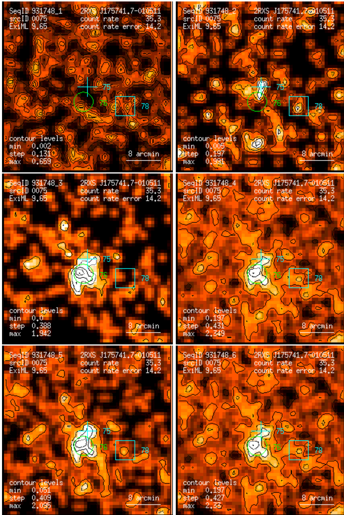
Figure 75: RASS 931748: detection 0075: band rate images, Gaussian filter: (1) PSPC channels 11 – 41, (2) 52 – 90, (3) 91 – 201, (4) 11 – 235, (5) 52 – 201, (6) 11 – 201. Broad band rates in counts/ks. Band rate contour levels in counts/ks/arcmin 2 .
