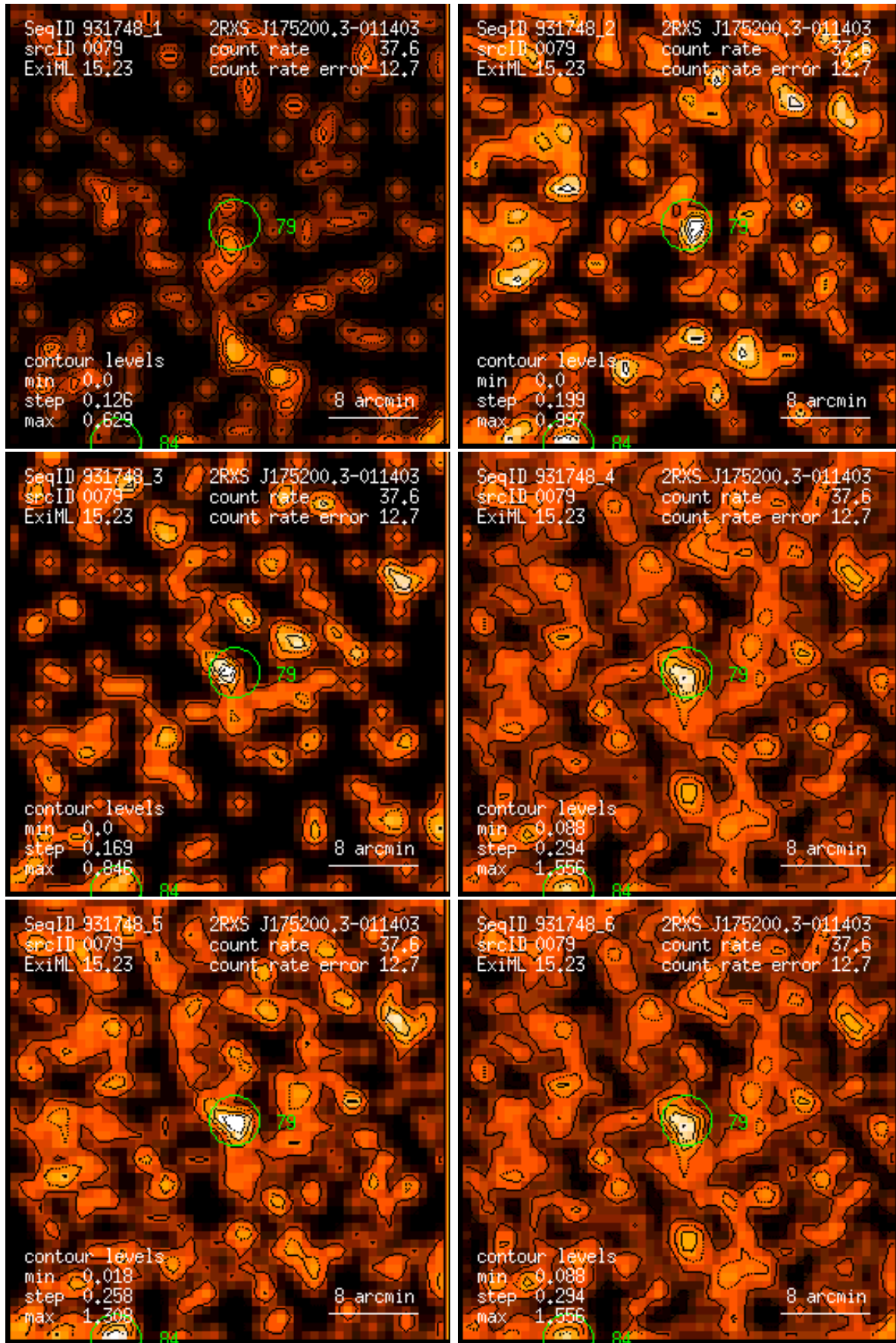
Figure 79: RASS 931748: detection 0079: band rate images, Gaussian filter: (1) PSPC channels 11 – 41, (2) 52 – 90, (3) 91 – 201, (4) 11 – 235, (5) 52 – 201, (6) 11 – 201. Broad band rates in counts/ks. Band rate contour levels in counts/ks/arcmin 2 .
