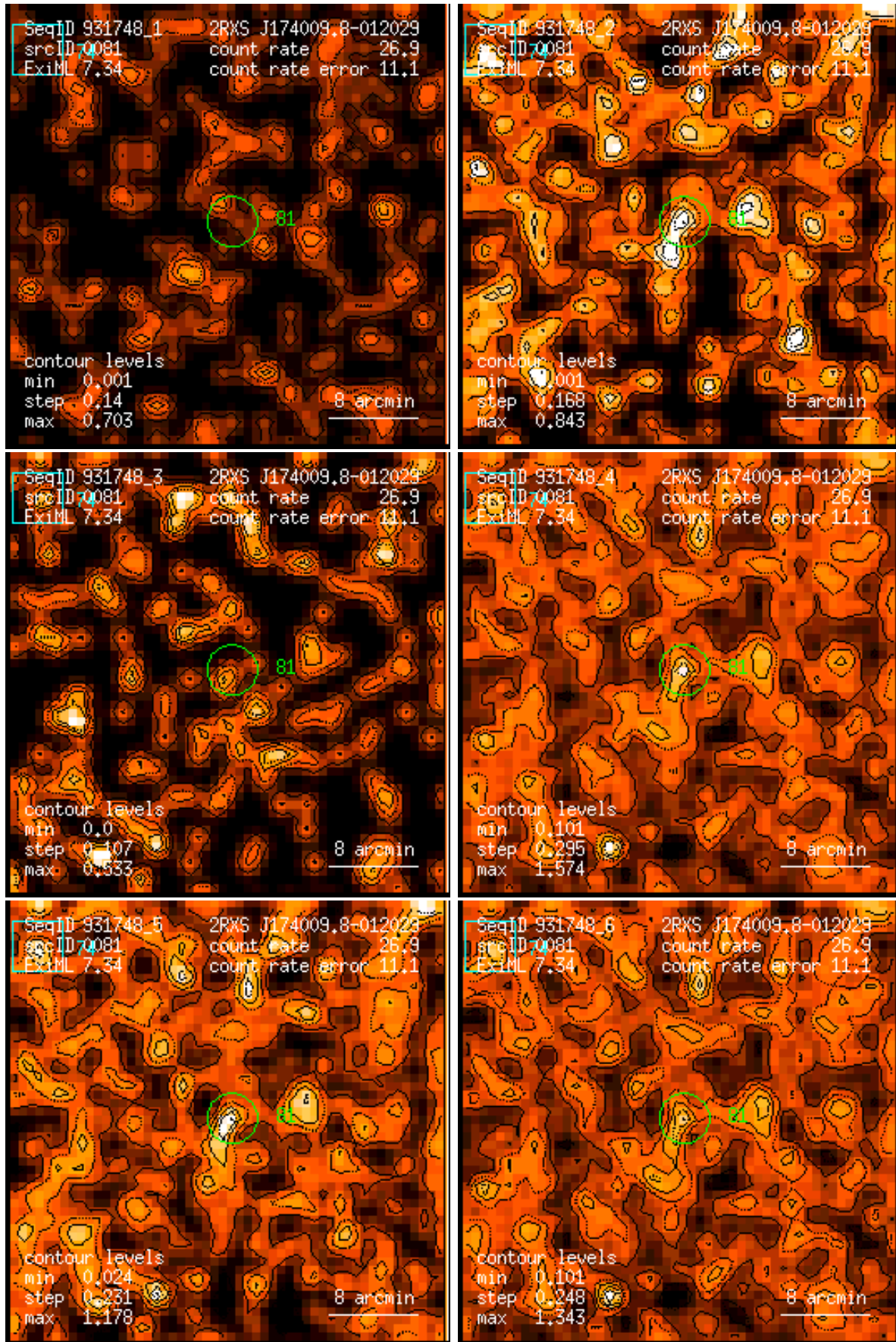
Figure 81: RASS 931748: detection 0081: band rate images, Gaussian filter: (1) PSPC channels 11 – 41, (2) 52 – 90, (3) 91 – 201, (4) 11 – 235, (5) 52 – 201, (6) 11 – 201. Broad band rates in counts/ks. Band rate contour levels in counts/ks/arcmin 2 .
