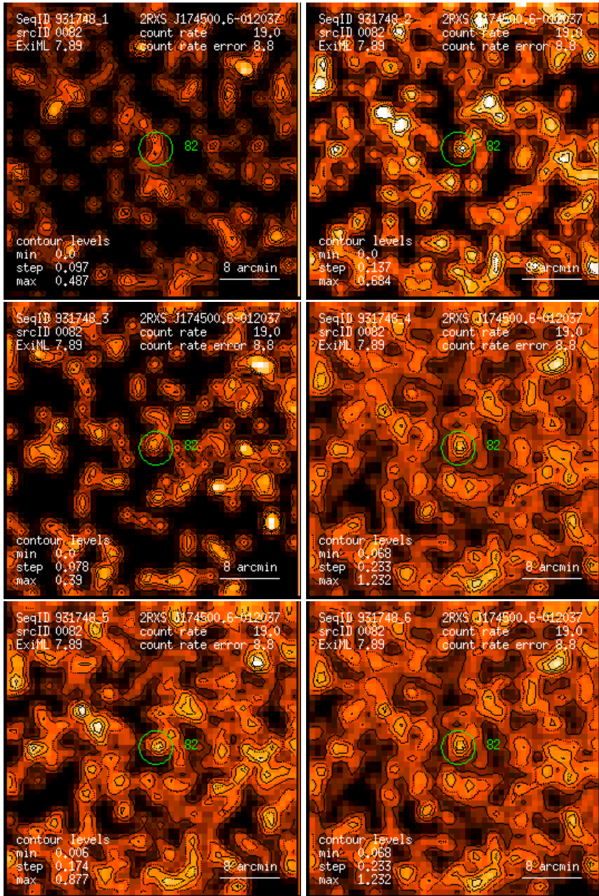
Figure 82: RASS 931748: detection 0082: band rate images, Gaussian filter: (1) PSPC channels 11 – 41, (2) 52 – 90, (3) 91 – 201, (4) 11 – 235, (5) 52 – 201, (6) 11 – 201. Broad band rates in counts/ks. Band rate contour levels in counts/ks/arcmin 2 .
