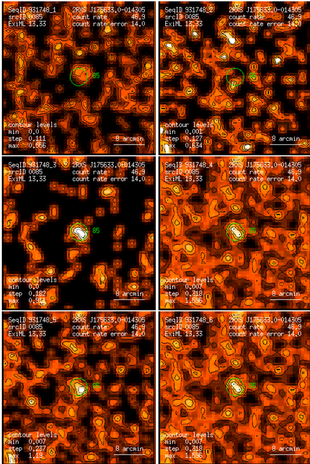
Figure 85: RASS 931748: detection 0085: band rate images, Gaussian filter: (1) PSPC channels 11 – 41, (2) 52 – 90, (3) 91 – 201, (4) 11 – 235, (5) 52 – 201, (6) 11 – 201. Broad band rates in counts/ks. Band rate contour levels in counts/ks/arcmin 2 .
