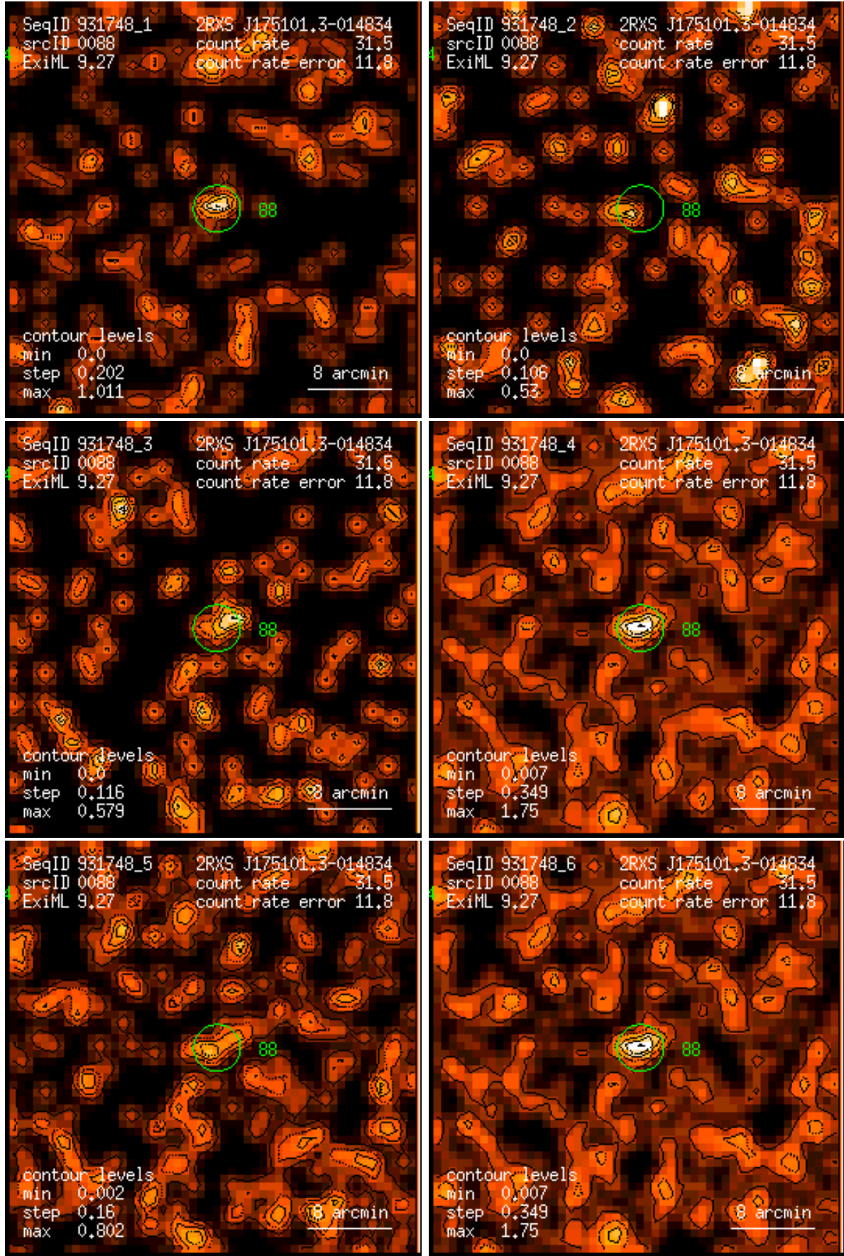
Figure 88: RASS 931748: detection 0088: band rate images, Gaussian filter: (1) PSPC channels 11 – 41, (2) 52 – 90, (3) 91 – 201, (4) 11 – 235, (5) 52 – 201, (6) 11 – 201. Broad band rates in counts/ks. Band rate contour levels in counts/ks/arcmin 2 .
