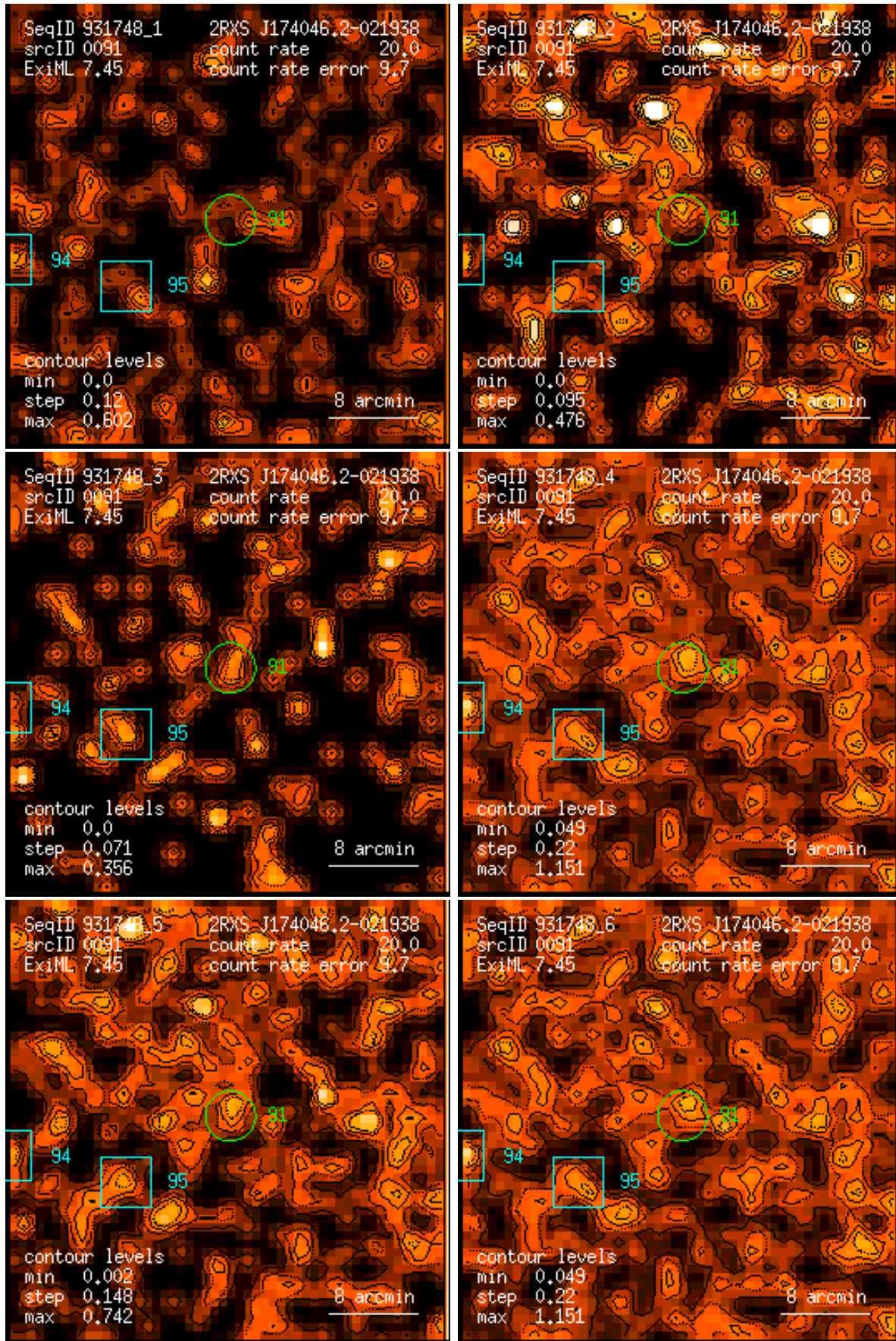
Figure 91: RASS 931748: detection 0091: band rate images, Gaussian filter: (1) PSPC channels 11 – 41, (2) 52 – 90, (3) 91 – 201, (4) 11 – 235, (5) 52 – 201, (6) 11 – 201. Broad band rates in counts/ks. Band rate contour levels in counts/ks/arcmin 2 .
