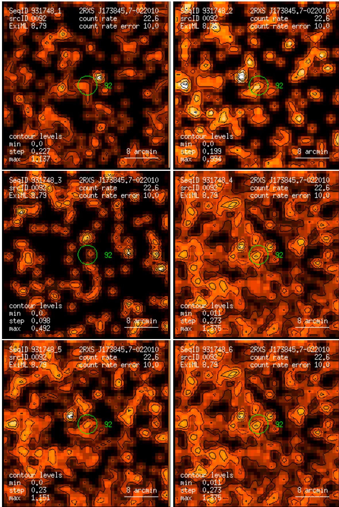
Figure 92: RASS 931748: detection 0092: band rate images, Gaussian filter: (1) PSPC channels 11 – 41, (2) 52 – 90, (3) 91 – 201, (4) 11 – 235, (5) 52 – 201, (6) 11 – 201. Broad band rates in counts/ks. Band rate contour levels in counts/ks/arcmin 2 .
