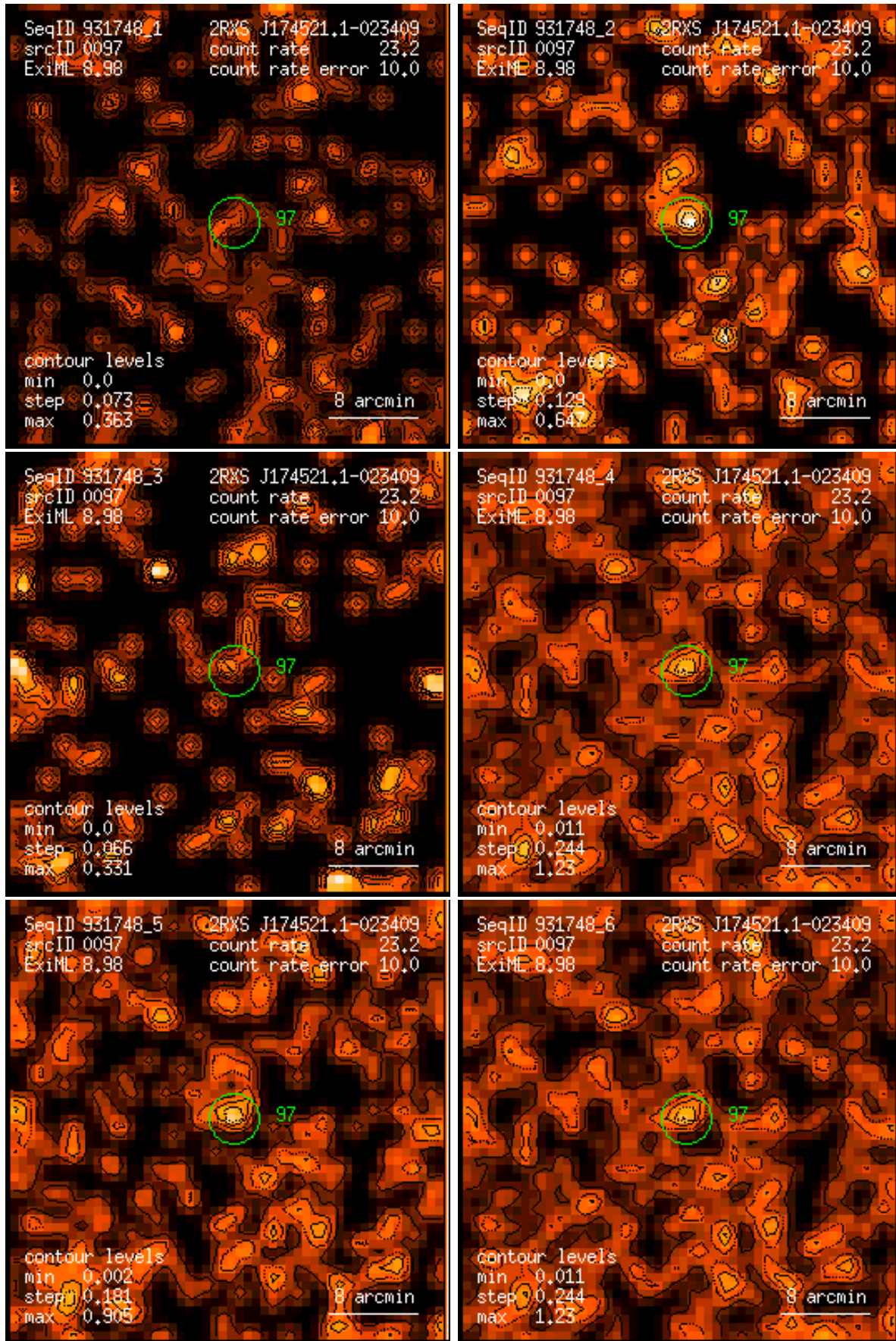
Figure 97: RASS 931748: detection 0097: band rate images, Gaussian filter: (1) PSPC channels 11 – 41, (2) 52 – 90, (3) 91 – 201, (4) 11 – 235, (5) 52 – 201, (6) 11 – 201. Broad band rates in counts/ks. Band rate contour levels in counts/ks/arcmin 2 .
