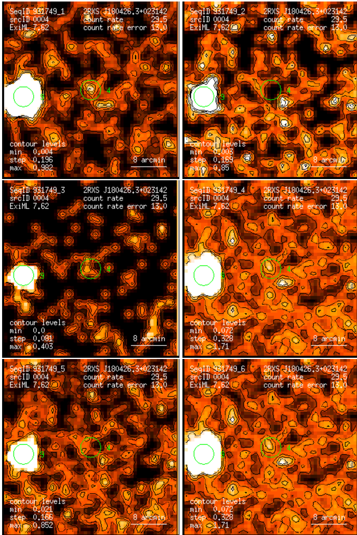
Figure 4: RASS 931749: detection 0004: band rate images, Gaussian filter: (1) PSPC channels 11 – 41, (2) 52 – 90, (3) 91 – 201, (4) 11 – 235, (5) 52 – 201, (6) 11 – 201. Broad band rates in counts/ks. Band rate contour levels in counts/ks/arcmin 2 .
