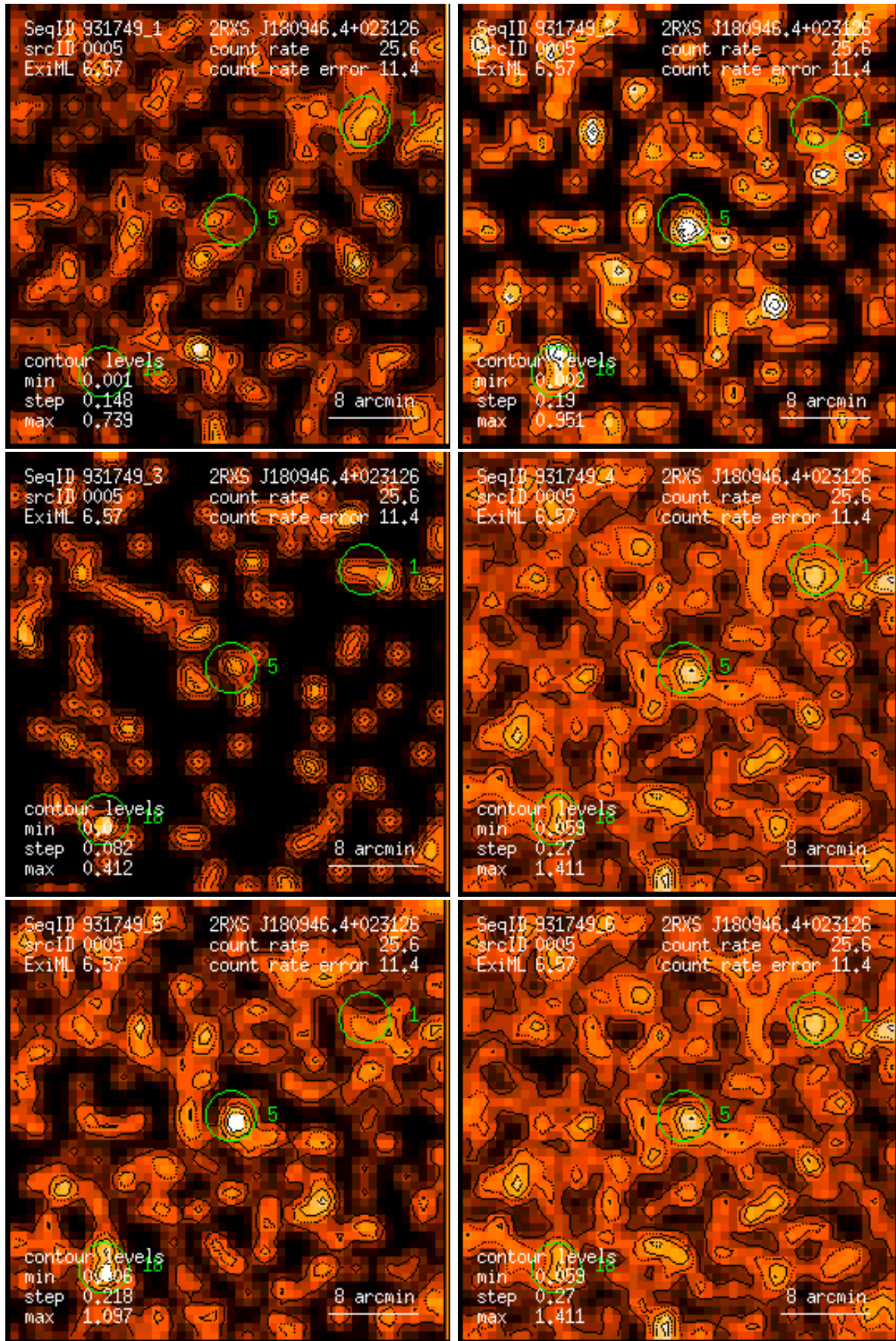
Figure 5: RASS 931749: detection 0005: band rate images, Gaussian filter: (1) PSPC channels 11 – 41, (2) 52 – 90, (3) 91 – 201, (4) 11 – 235, (5) 52 – 201, (6) 11 – 201. Broad band rates in counts/ks. Band rate contour levels in counts/ks/arcmin 2 .
