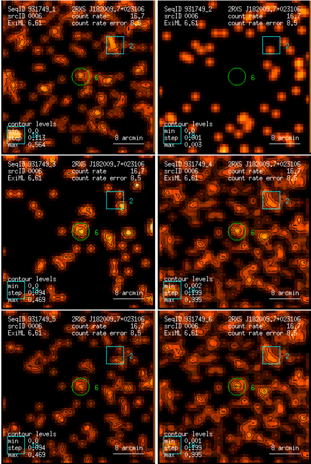
Figure 6: RASS 931749: detection 0006: band rate images, Gaussian filter: (1) PSPC channels 11 – 41, (2) 52 – 90, (3) 91 – 201, (4) 11 – 235, (5) 52 – 201, (6) 11 – 201. Broad band rates in counts/ks. Band rate contour levels in counts/ks/arcmin 2 .
