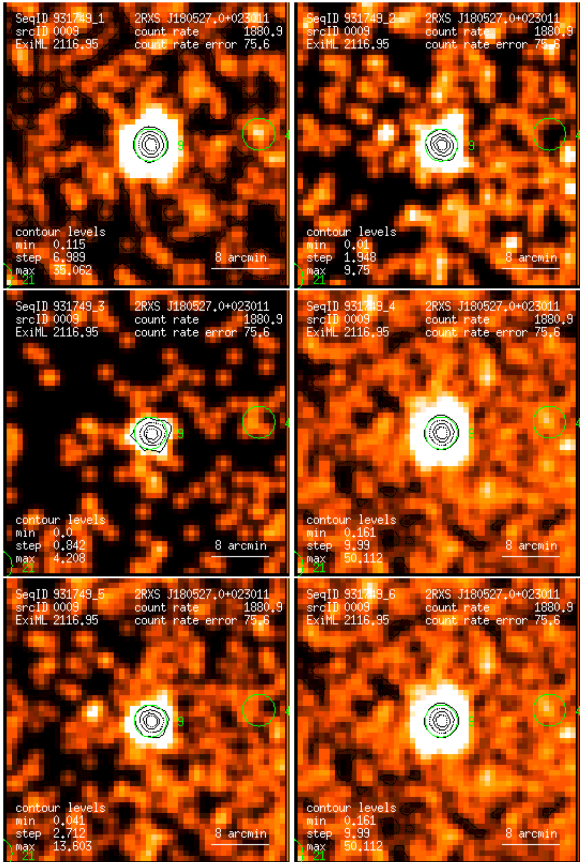
Figure 9: RASS 931749: detection 0009: band rate images, Gaussian filter: (1) PSPC channels 11 – 41, (2) 52 – 90, (3) 91 – 201, (4) 11 – 235, (5) 52 – 201, (6) 11 – 201. Broad band rates in counts/ks. Band rate contour levels in counts/ks/arcmin 2 .
