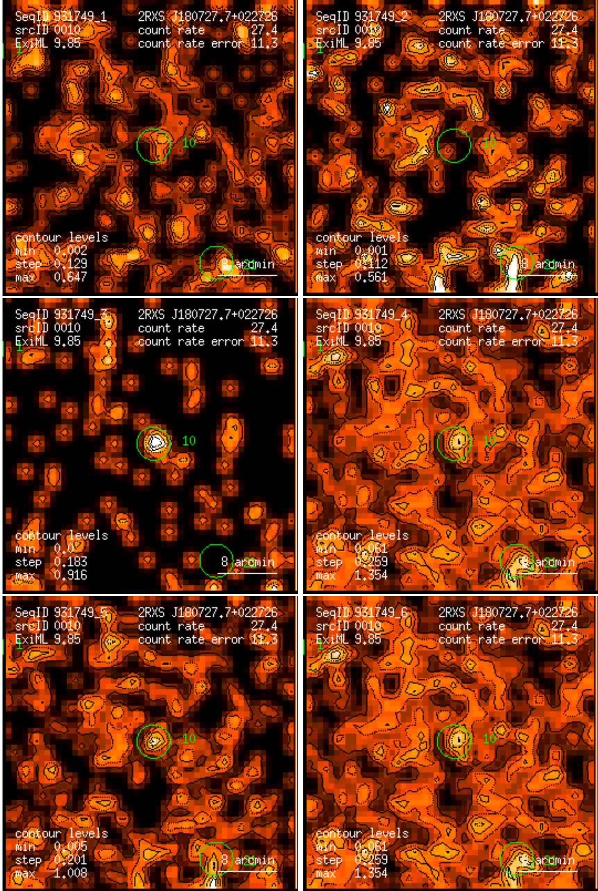
Figure 10: RASS 931749: detection 0010: band rate images, Gaussian filter: (1) PSPC channels 11 – 41, (2) 52 – 90, (3) 91 – 201, (4) 11 – 235, (5) 52 – 201, (6) 11 – 201. Broad band rates in counts/ks. Band rate contour levels in counts/ks/arcmin 2 .
