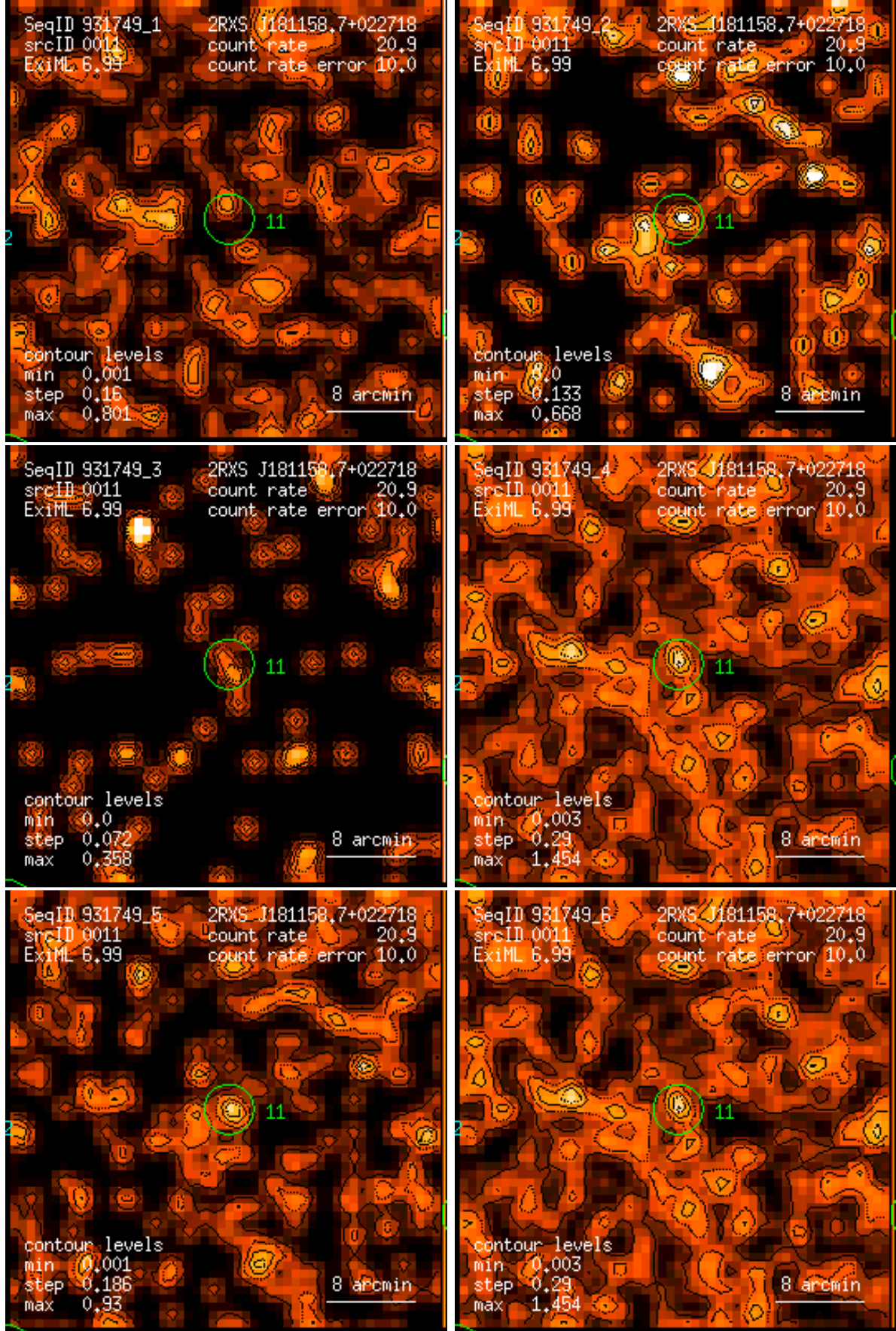
Figure 11: RASS 931749: detection 0011: band rate images, Gaussian filter: (1) PSPC channels 11 – 41, (2) 52 – 90, (3) 91 – 201, (4) 11 – 235, (5) 52 – 201, (6) 11 – 201. Broad band rates in counts/ks. Band rate contour levels in counts/ks/arcmin 2 .
