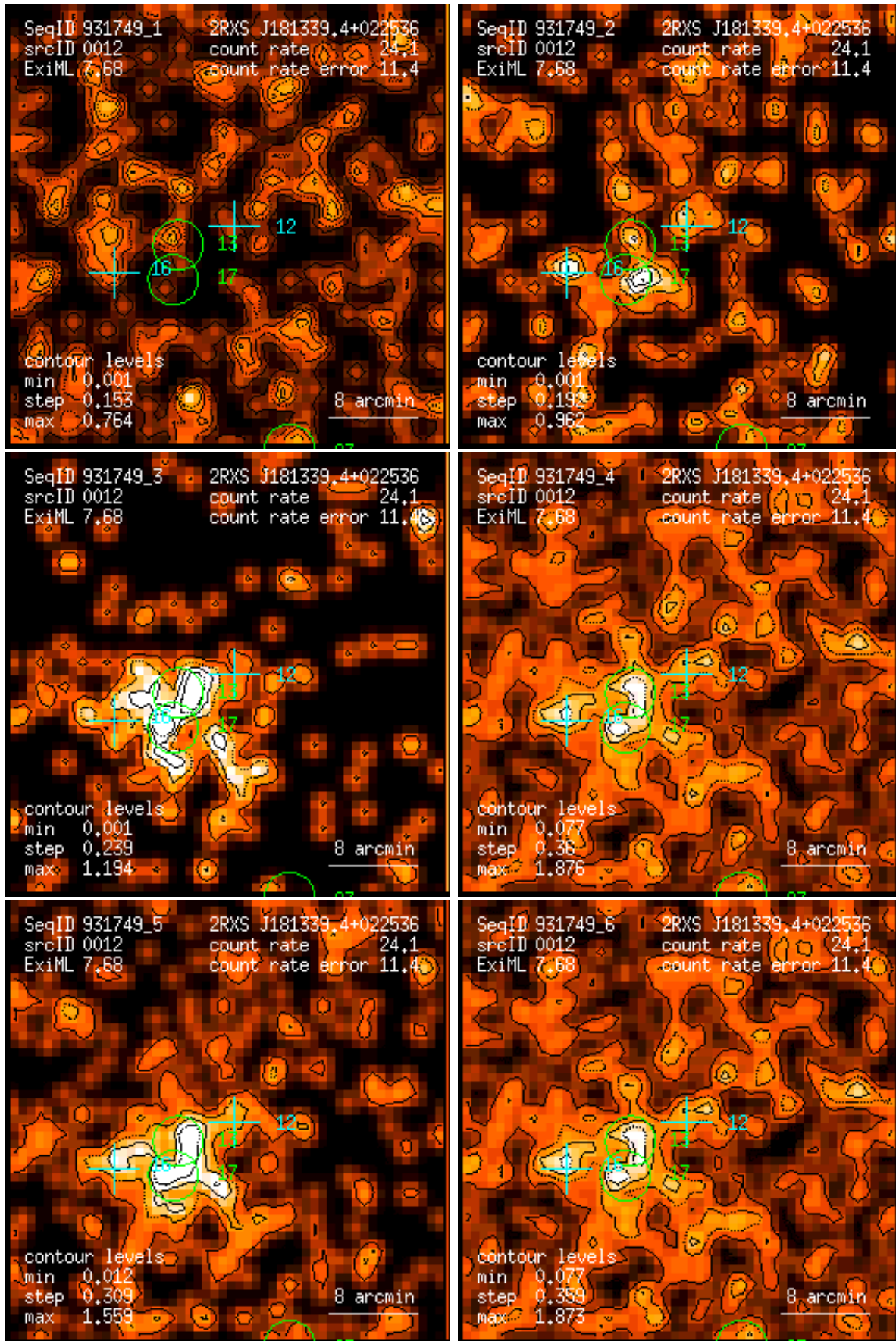
Figure 12: RASS 931749: detection 0012: band rate images, Gaussian filter: (1) PSPC channels 11 – 41, (2) 52 – 90, (3) 91 – 201, (4) 11 – 235, (5) 52 – 201, (6) 11 – 201. Broad band rates in counts/ks. Band rate contour levels in counts/ks/arcmin 2 .
