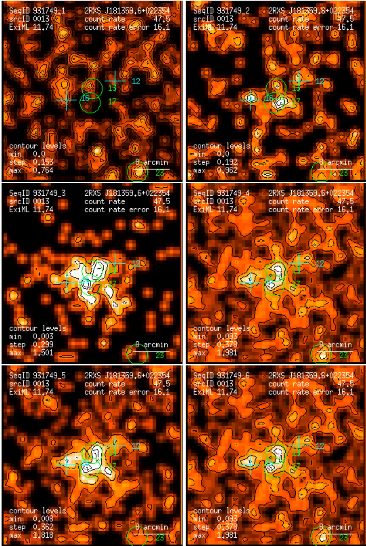
Figure 13: RASS 931749: detection 0013: band rate images, Gaussian filter: (1) PSPC channels 11 – 41, (2) 52 – 90, (3) 91 – 201, (4) 11 – 235, (5) 52 – 201, (6) 11 – 201. Broad band rates in counts/ks. Band rate contour levels in counts/ks/arcmin 2 .
