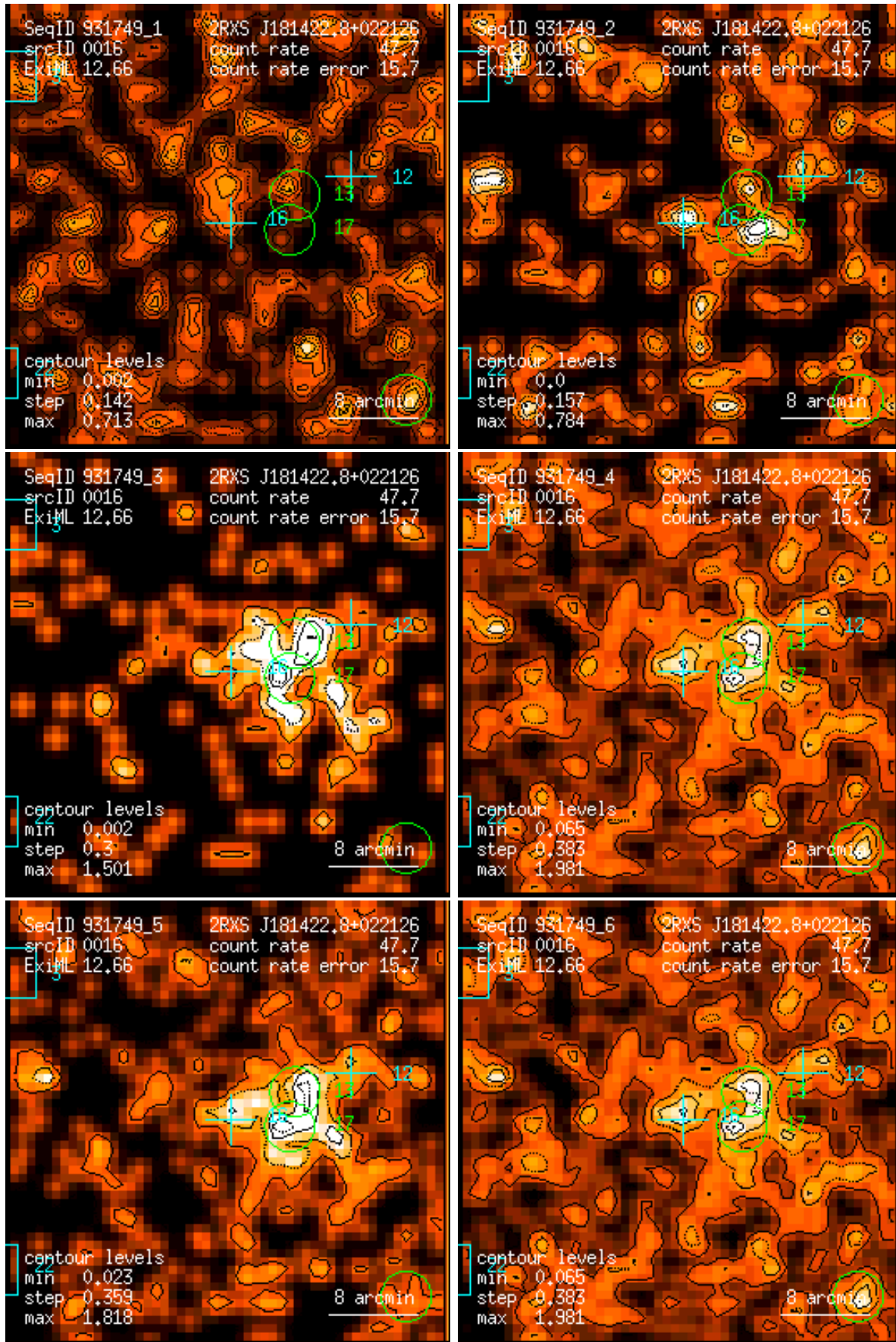
Figure 16: RASS 931749: detection 0016: band rate images, Gaussian filter: (1) PSPC channels 11 – 41, (2) 52 – 90, (3) 91 – 201, (4) 11 – 235, (5) 52 – 201, (6) 11 – 201. Broad band rates in counts/ks. Band rate contour levels in counts/ks/arcmin 2 .
