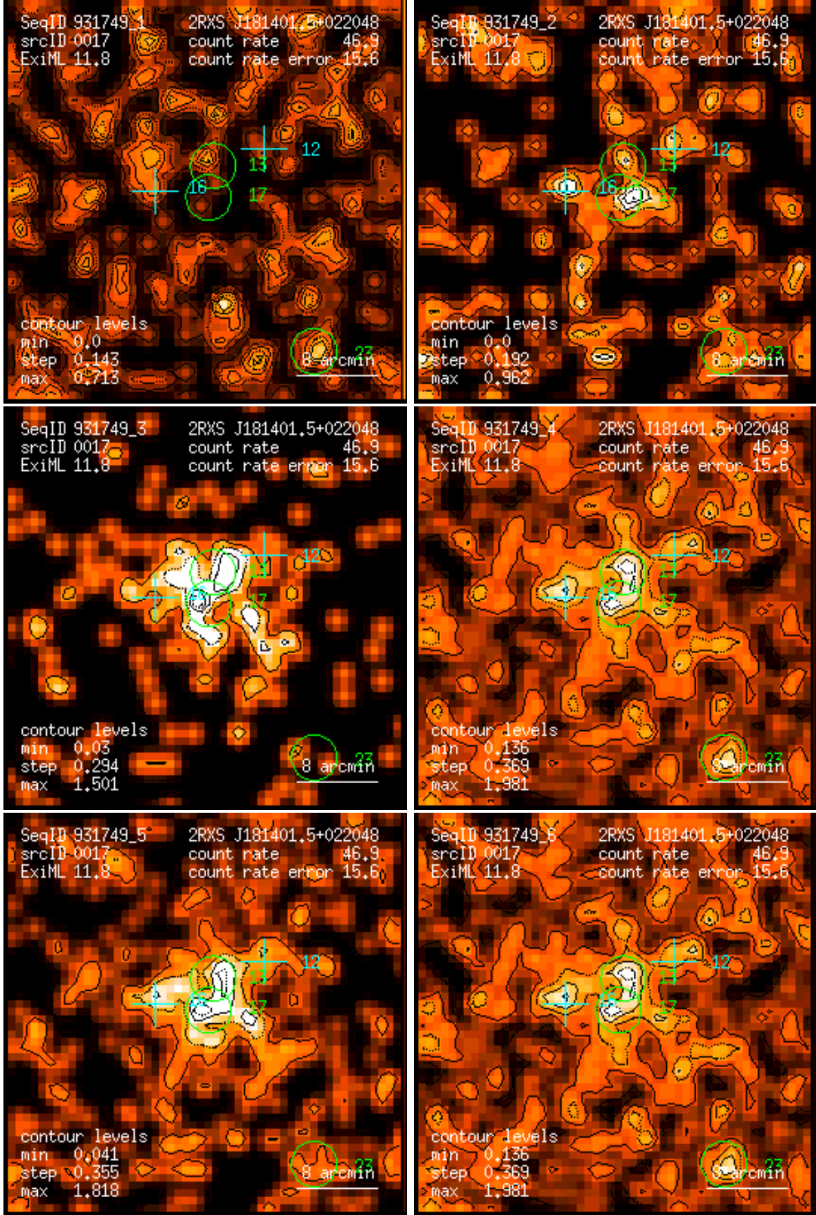
Figure 17: RASS 931749: detection 0017: band rate images, Gaussian filter: (1) PSPC channels 11 – 41, (2) 52 – 90, (3) 91 – 201, (4) 11 – 235, (5) 52 – 201, (6) 11 – 201. Broad band rates in counts/ks. Band rate contour levels in counts/ks/arcmin 2 .
