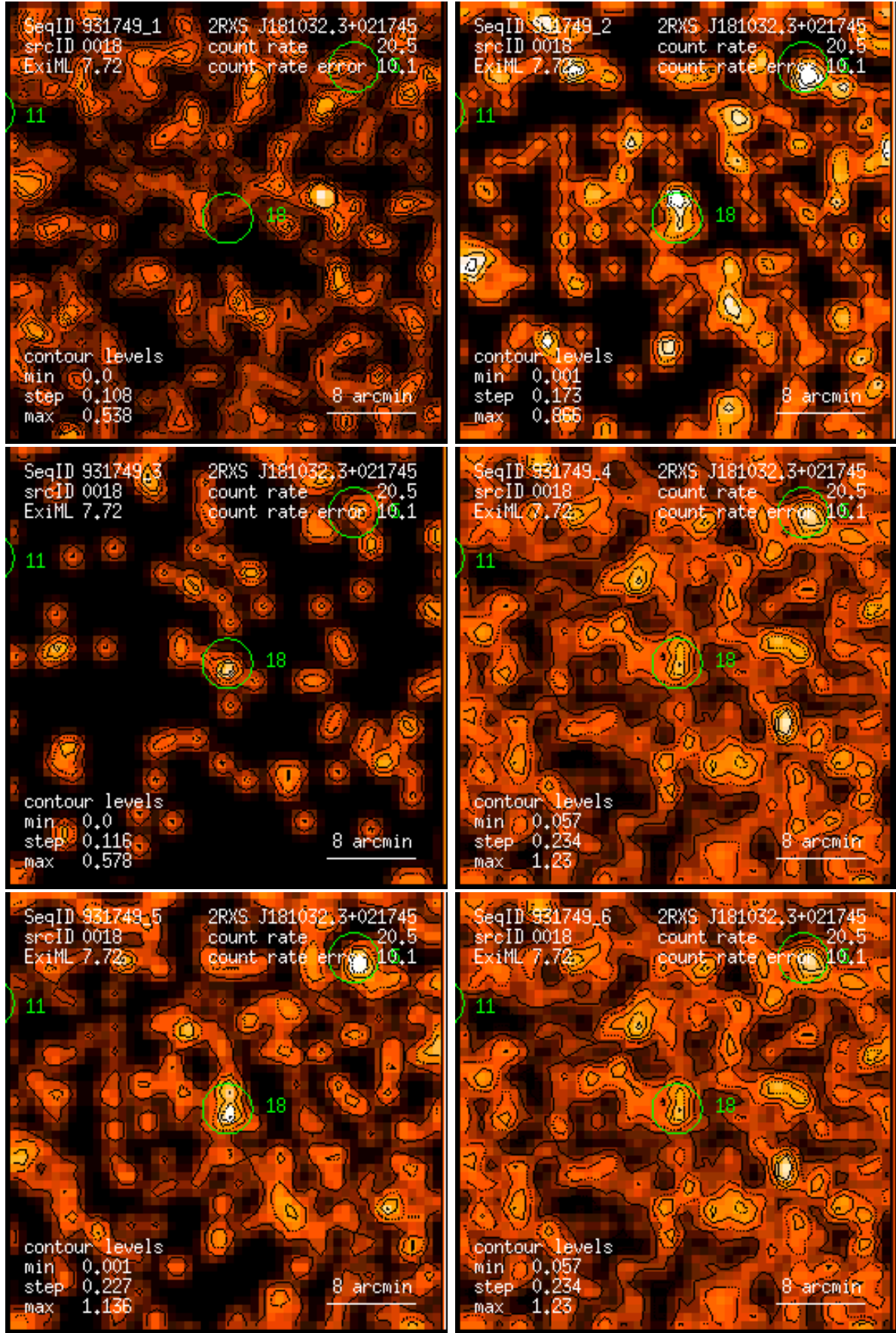
Figure 18: RASS 931749: detection 0018: band rate images, Gaussian filter: (1) PSPC channels 11 – 41, (2) 52 – 90, (3) 91 – 201, (4) 11 – 235, (5) 52 – 201, (6) 11 – 201. Broad band rates in counts/ks. Band rate contour levels in counts/ks/arcmin 2 .
