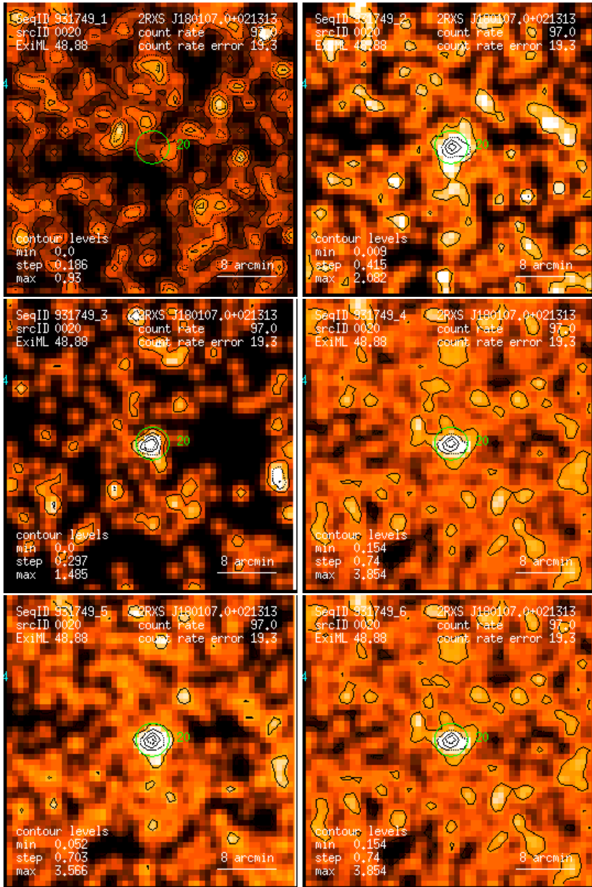
Figure 20: RASS 931749: detection 0020: band rate images, Gaussian filter: (1) PSPC channels 11 – 41, (2) 52 – 90, (3) 91 – 201, (4) 11 – 235, (5) 52 – 201, (6) 11 – 201. Broad band rates in counts/ks. Band rate contour levels in counts/ks/arcmin 2 .
