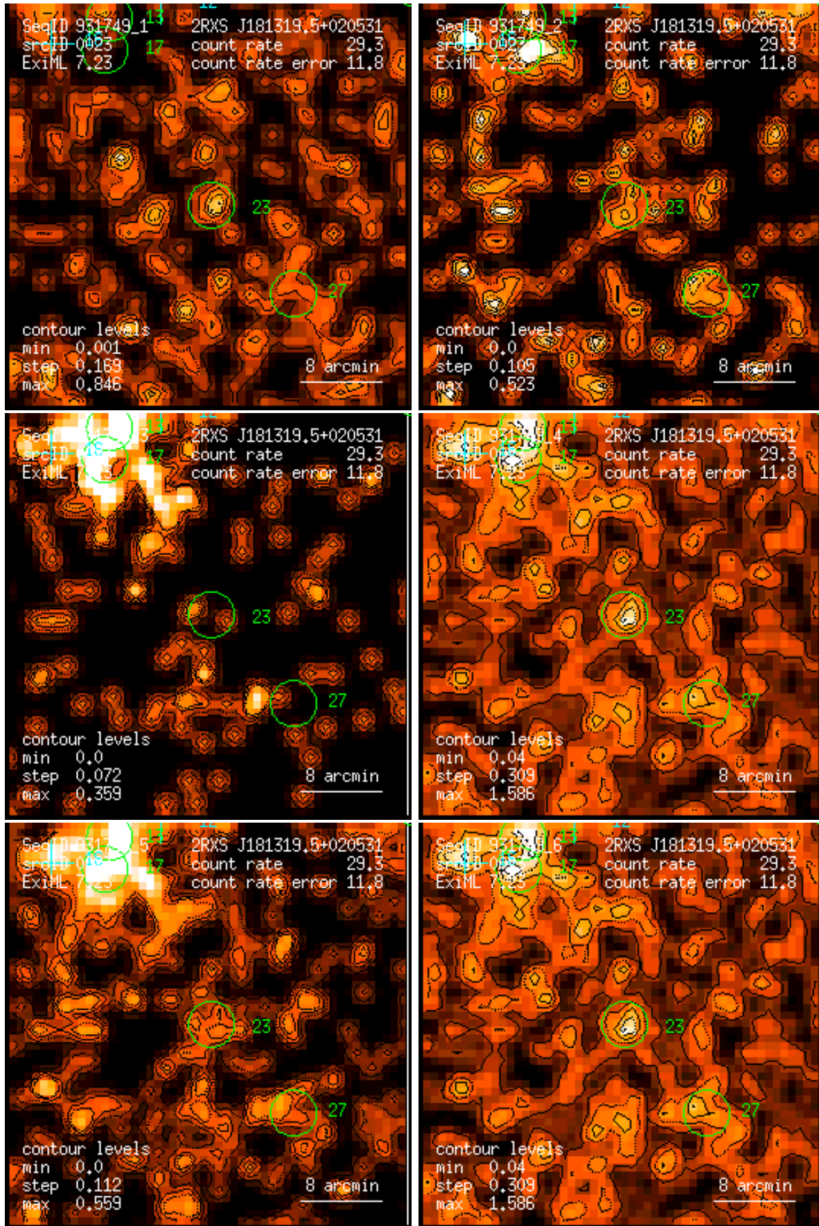
Figure 23: RASS 931749: detection 0023: band rate images, Gaussian filter: (1) PSPC channels 11 – 41, (2) 52 – 90, (3) 91 – 201, (4) 11 – 235, (5) 52 – 201, (6) 11 – 201. Broad band rates in counts/ks. Band rate contour levels in counts/ks/arcmin 2 .
