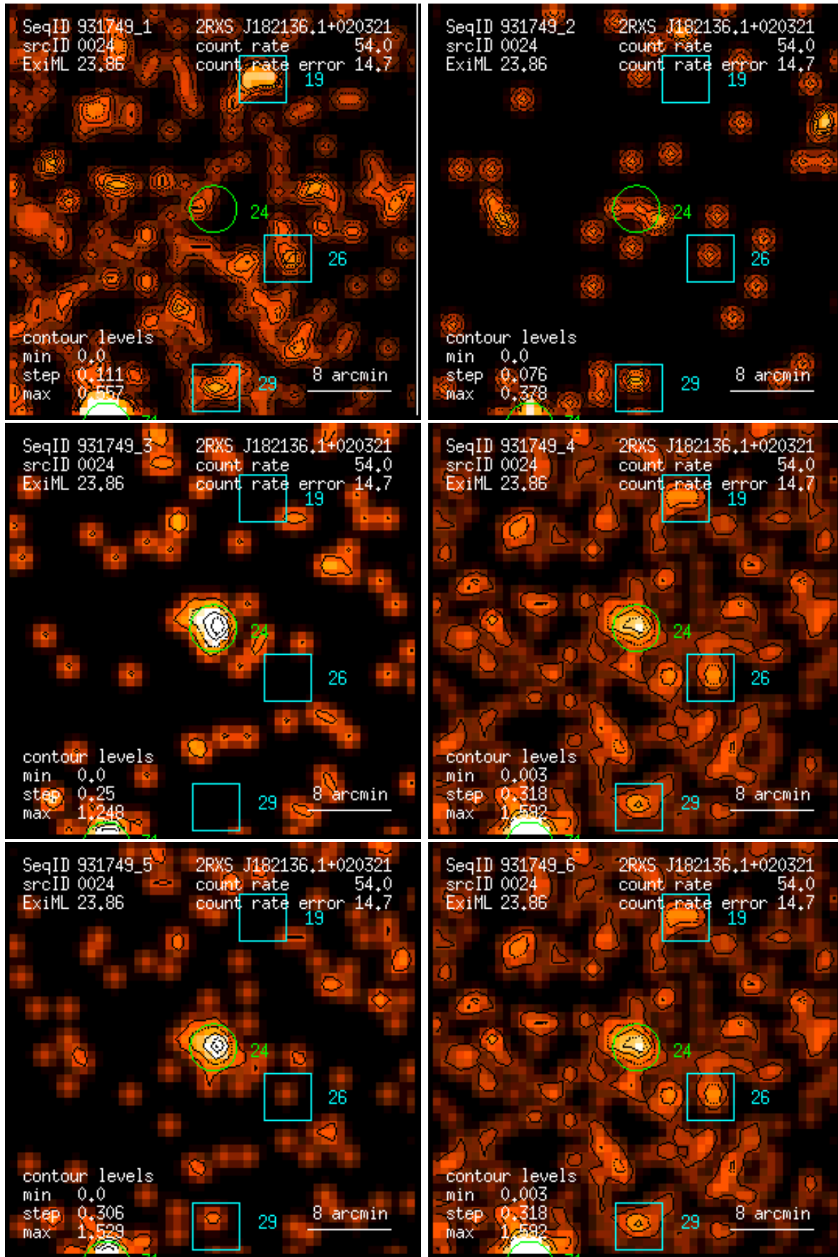
Figure 24: RASS 931749: detection 0024: band rate images, Gaussian filter: (1) PSPC channels 11 – 41, (2) 52 – 90, (3) 91 – 201, (4) 11 – 235, (5) 52 – 201, (6) 11 – 201. Broad band rates in counts/ks. Band rate contour levels in counts/ks/arcmin 2 .
