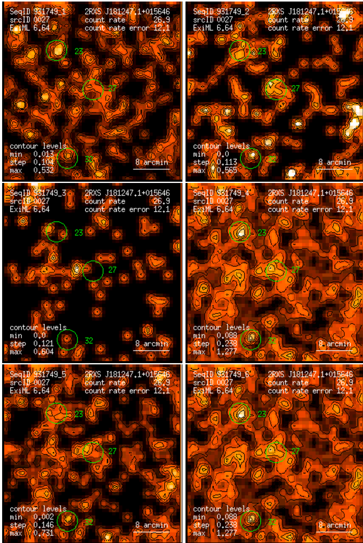
Figure 27: RASS 931749: detection 0027: band rate images, Gaussian filter: (1) PSPC channels 11 – 41, (2) 52 – 90, (3) 91 – 201, (4) 11 – 235, (5) 52 – 201, (6) 11 – 201. Broad band rates in counts/ks. Band rate contour levels in counts/ks/arcmin 2 .
