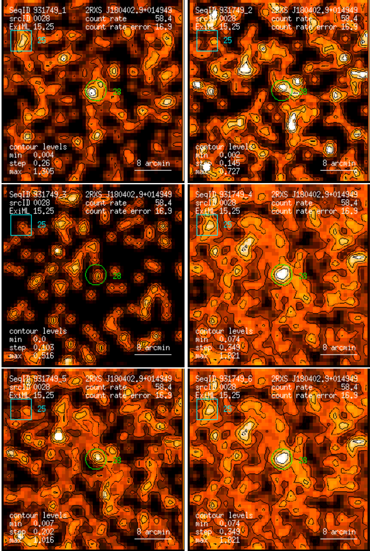
Figure 28: RASS 931749: detection 0028: band rate images, Gaussian filter: (1) PSPC channels 11 – 41, (2) 52 – 90, (3) 91 – 201, (4) 11 – 235, (5) 52 – 201, (6) 11 – 201. Broad band rates in counts/ks. Band rate contour levels in counts/ks/arcmin 2 .
