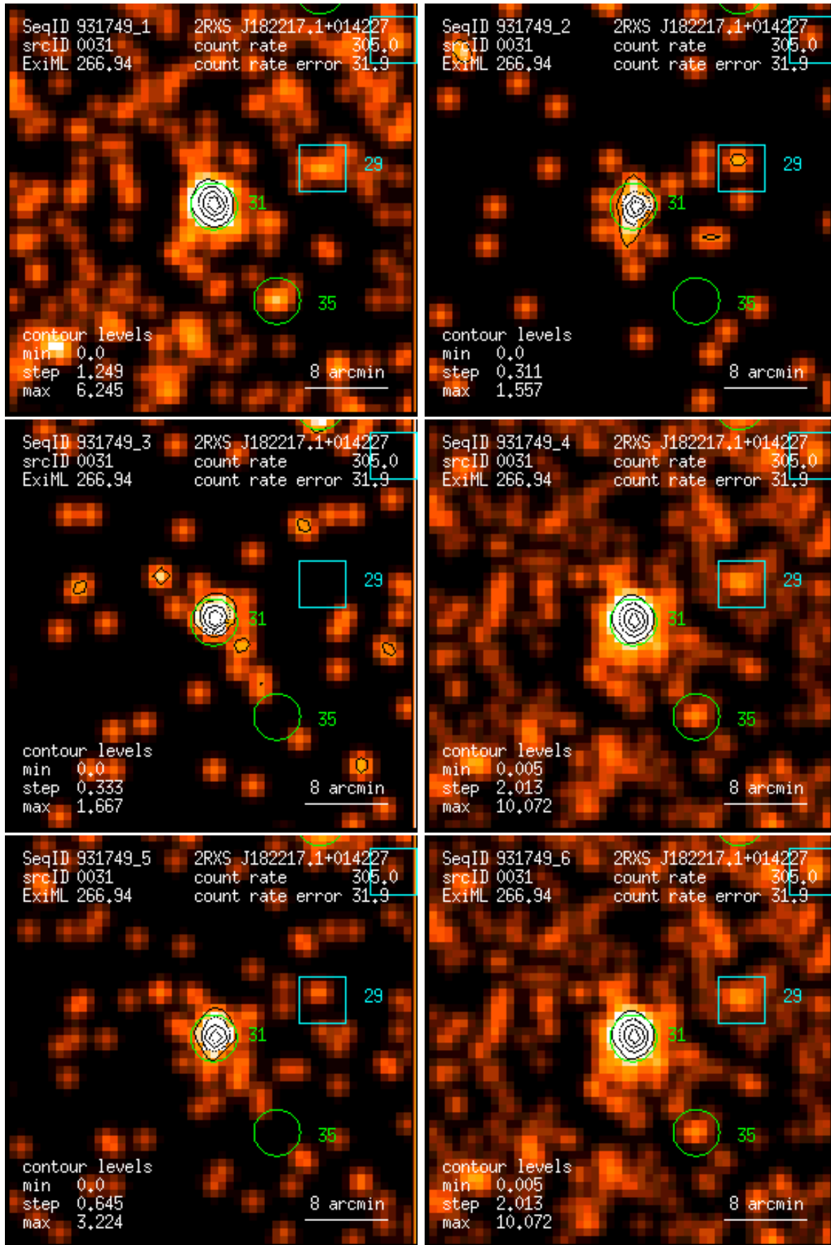
Figure 31: RASS 931749: detection 0031: band rate images, Gaussian filter: (1) PSPC channels 11 – 41, (2) 52 – 90, (3) 91 – 201, (4) 11 – 235, (5) 52 – 201, (6) 11 – 201. Broad band rates in counts/ks. Band rate contour levels in counts/ks/arcmin 2 .
