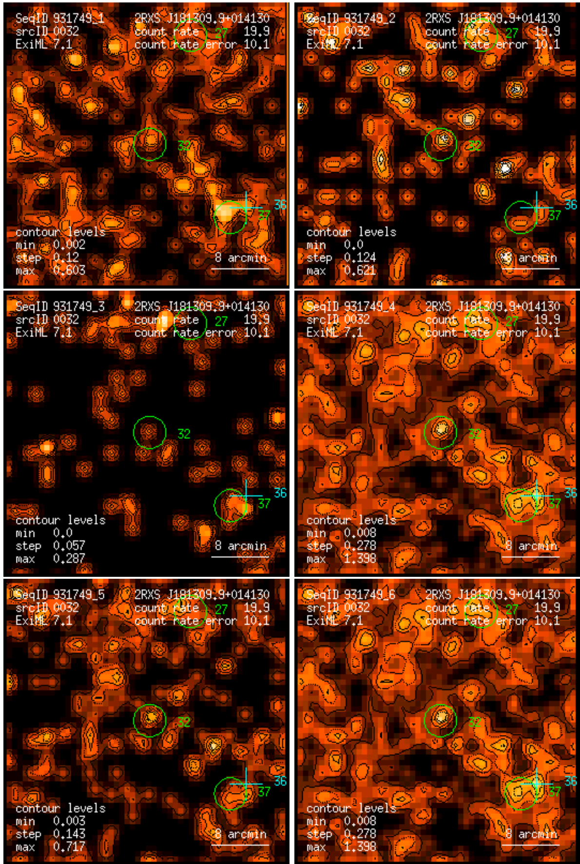
Figure 32: RASS 931749: detection 0032: band rate images, Gaussian filter: (1) PSPC channels 11 – 41, (2) 52 – 90, (3) 91 – 201, (4) 11 – 235, (5) 52 – 201, (6) 11 – 201. Broad band rates in counts/ks. Band rate contour levels in counts/ks/arcmin 2 .
