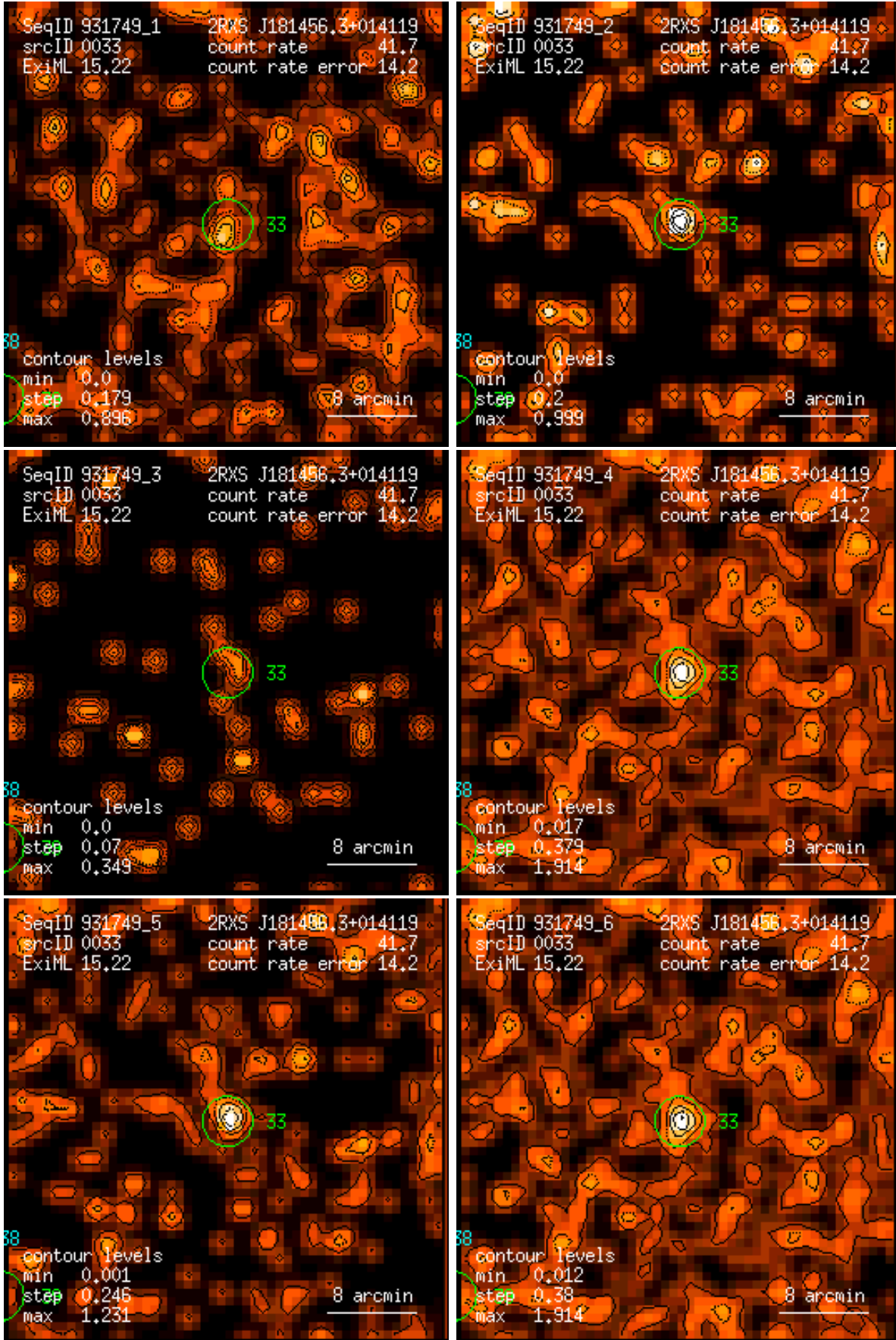
Figure 33: RASS 931749: detection 0033: band rate images, Gaussian filter: (1) PSPC channels 11 – 41, (2) 52 – 90, (3) 91 – 201, (4) 11 – 235, (5) 52 – 201, (6) 11 – 201. Broad band rates in counts/ks. Band rate contour levels in counts/ks/arcmin 2 .
