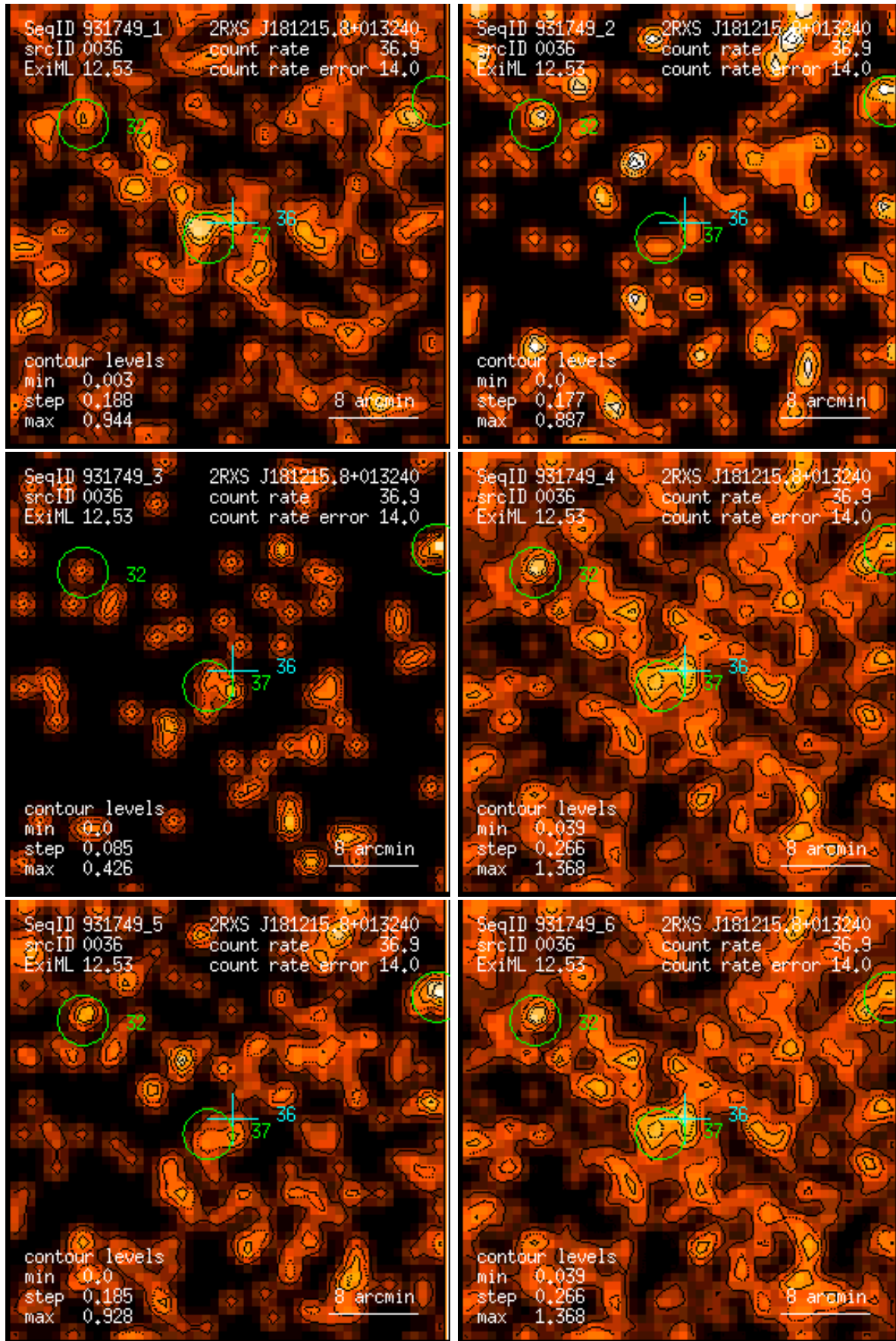
Figure 36: RASS 931749: detection 0036: band rate images, Gaussian filter: (1) PSPC channels 11 – 41, (2) 52 – 90, (3) 91 – 201, (4) 11 – 235, (5) 52 – 201, (6) 11 – 201. Broad band rates in counts/ks. Band rate contour levels in counts/ks/arcmin 2 .
