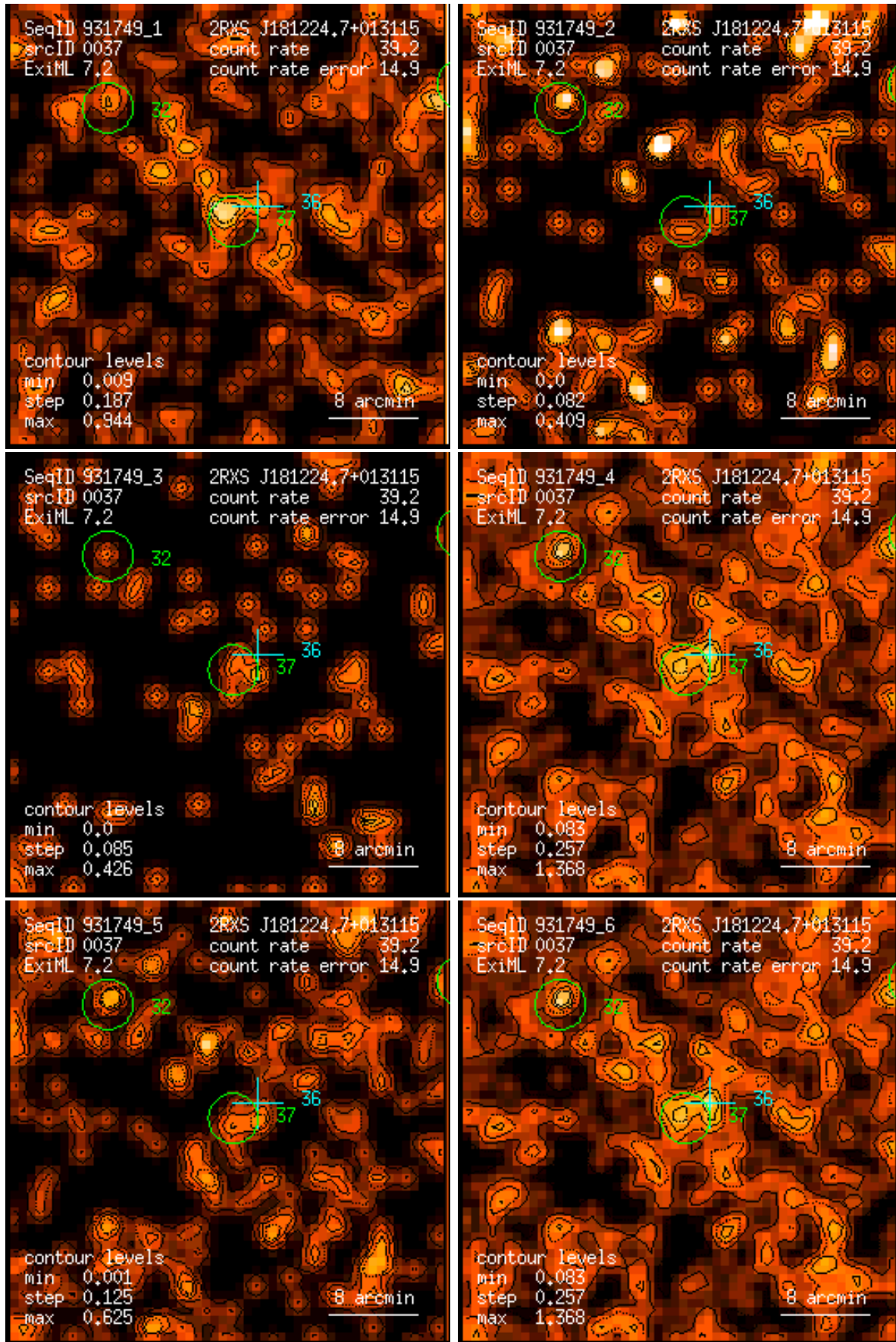
Figure 37: RASS 931749: detection 0037: band rate images, Gaussian filter: (1) PSPC channels 11 – 41, (2) 52 – 90, (3) 91 – 201, (4) 11 – 235, (5) 52 – 201, (6) 11 – 201. Broad band rates in counts/ks. Band rate contour levels in counts/ks/arcmin 2 .
