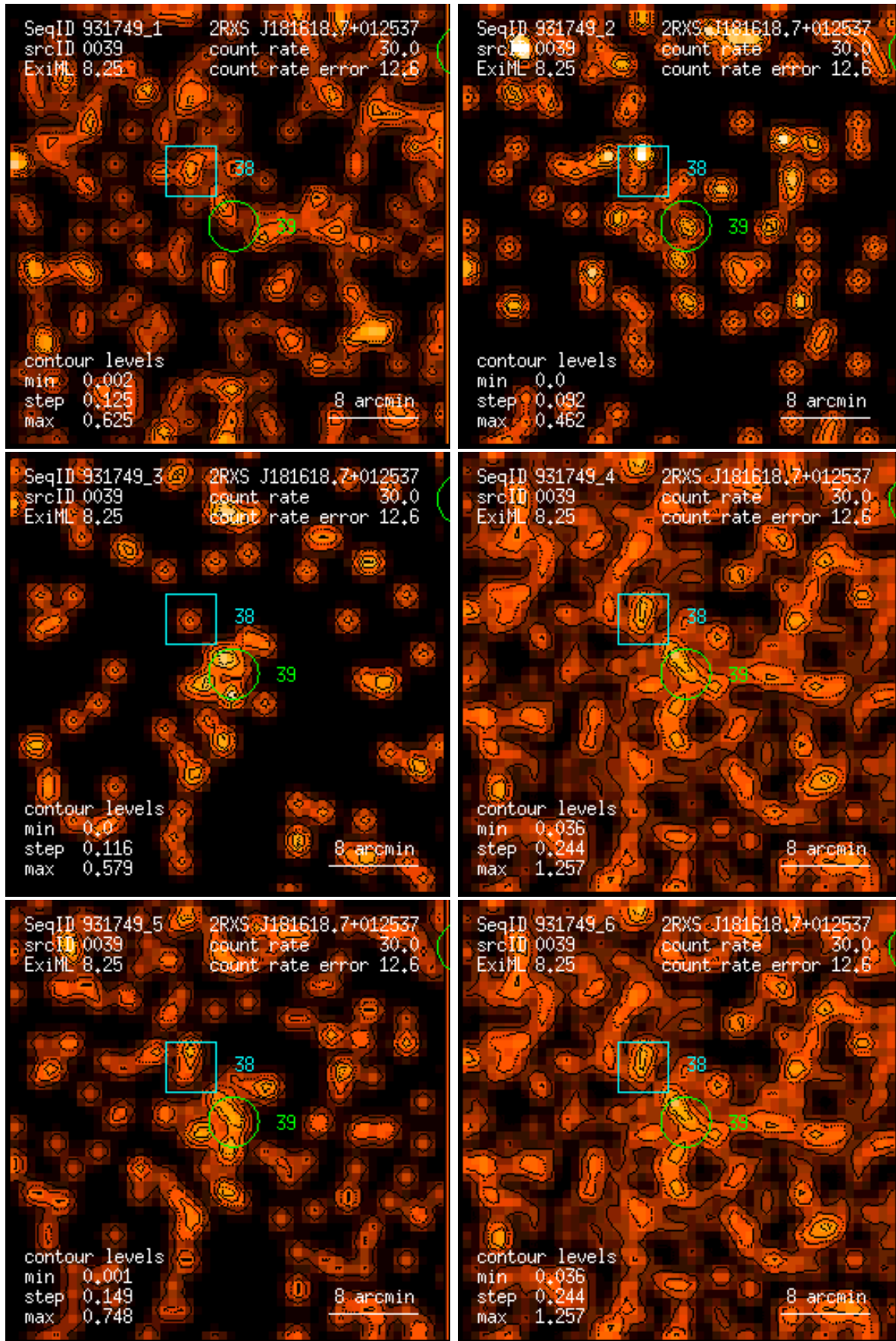
Figure 39: RASS 931749: detection 0039: band rate images, Gaussian filter: (1) PSPC channels 11 – 41, (2) 52 – 90, (3) 91 – 201, (4) 11 – 235, (5) 52 – 201, (6) 11 – 201. Broad band rates in counts/ks. Band rate contour levels in counts/ks/arcmin 2 .
