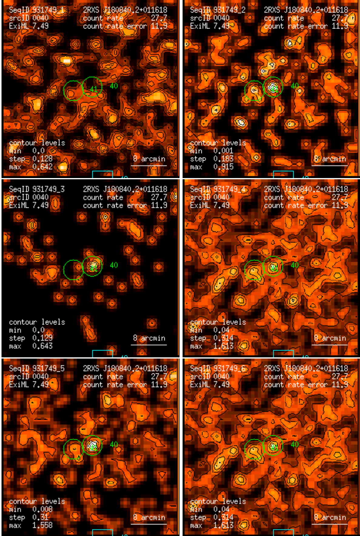
Figure 40: RASS 931749: detection 0040: band rate images, Gaussian filter: (1) PSPC channels 11 – 41, (2) 52 – 90, (3) 91 – 201, (4) 11 – 235, (5) 52 – 201, (6) 11 – 201. Broad band rates in counts/ks. Band rate contour levels in counts/ks/arcmin 2 .
