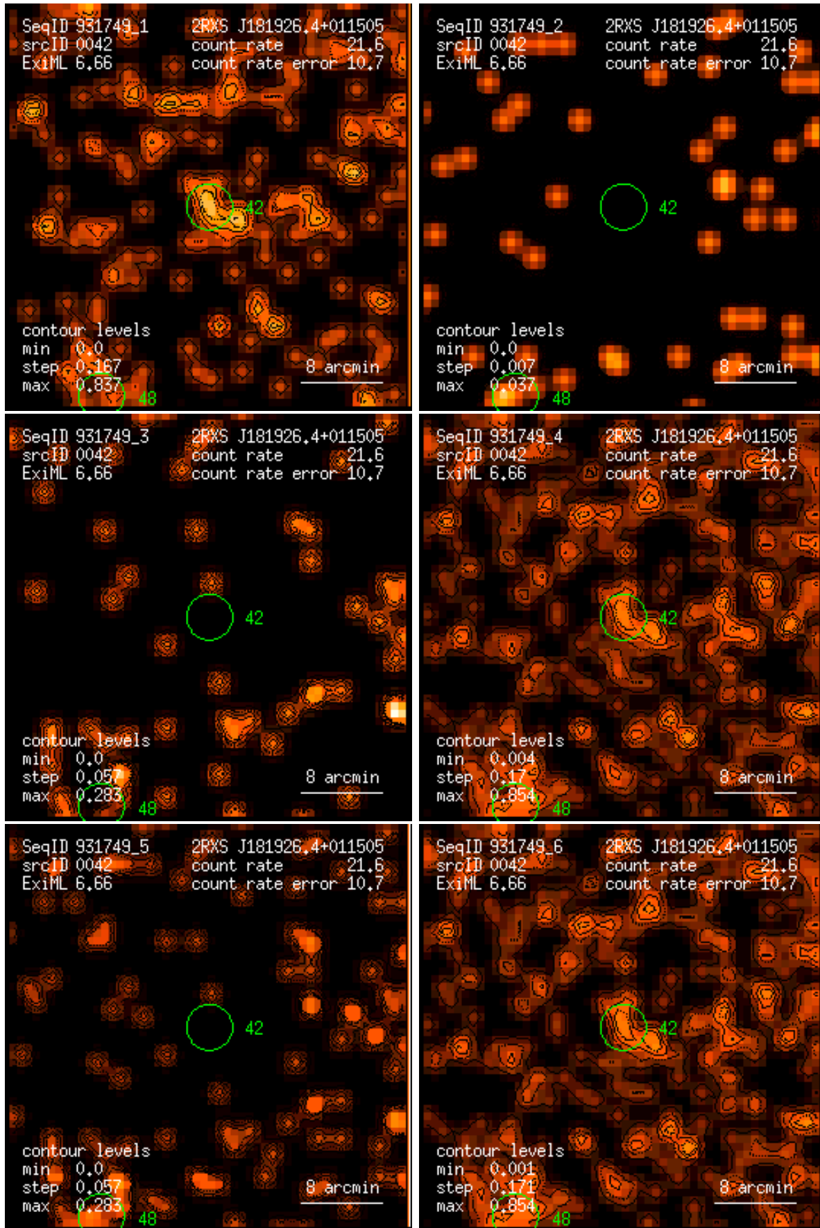
Figure 42: RASS 931749: detection 0042: band rate images, Gaussian filter: (1) PSPC channels 11 – 41, (2) 52 – 90, (3) 91 – 201, (4) 11 – 235, (5) 52 – 201, (6) 11 – 201. Broad band rates in counts/ks. Band rate contour levels in counts/ks/arcmin 2 .
