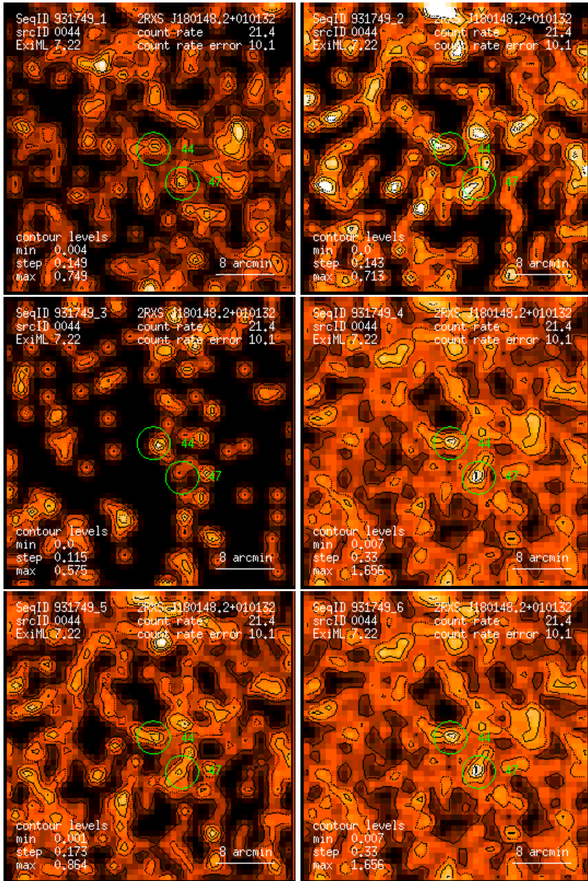
Figure 44: RASS 931749: detection 0044: band rate images, Gaussian filter: (1) PSPC channels 11 – 41, (2) 52 – 90, (3) 91 – 201, (4) 11 – 235, (5) 52 – 201, (6) 11 – 201. Broad band rates in counts/ks. Band rate contour levels in counts/ks/arcmin 2 .
