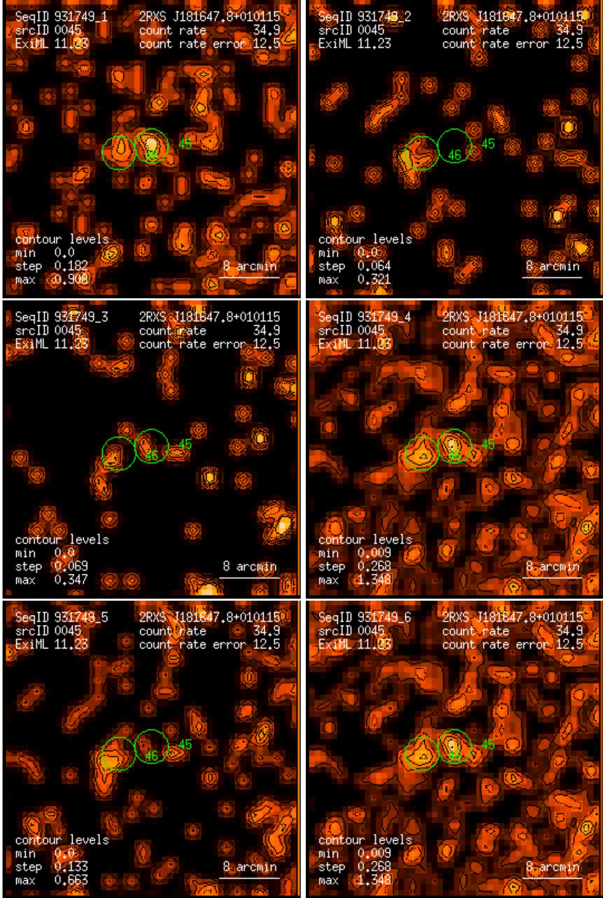
Figure 45: RASS 931749: detection 0045: band rate images, Gaussian filter: (1) PSPC channels 11 – 41, (2) 52 – 90, (3) 91 – 201, (4) 11 – 235, (5) 52 – 201, (6) 11 – 201. Broad band rates in counts/ks. Band rate contour levels in counts/ks/arcmin 2 .
