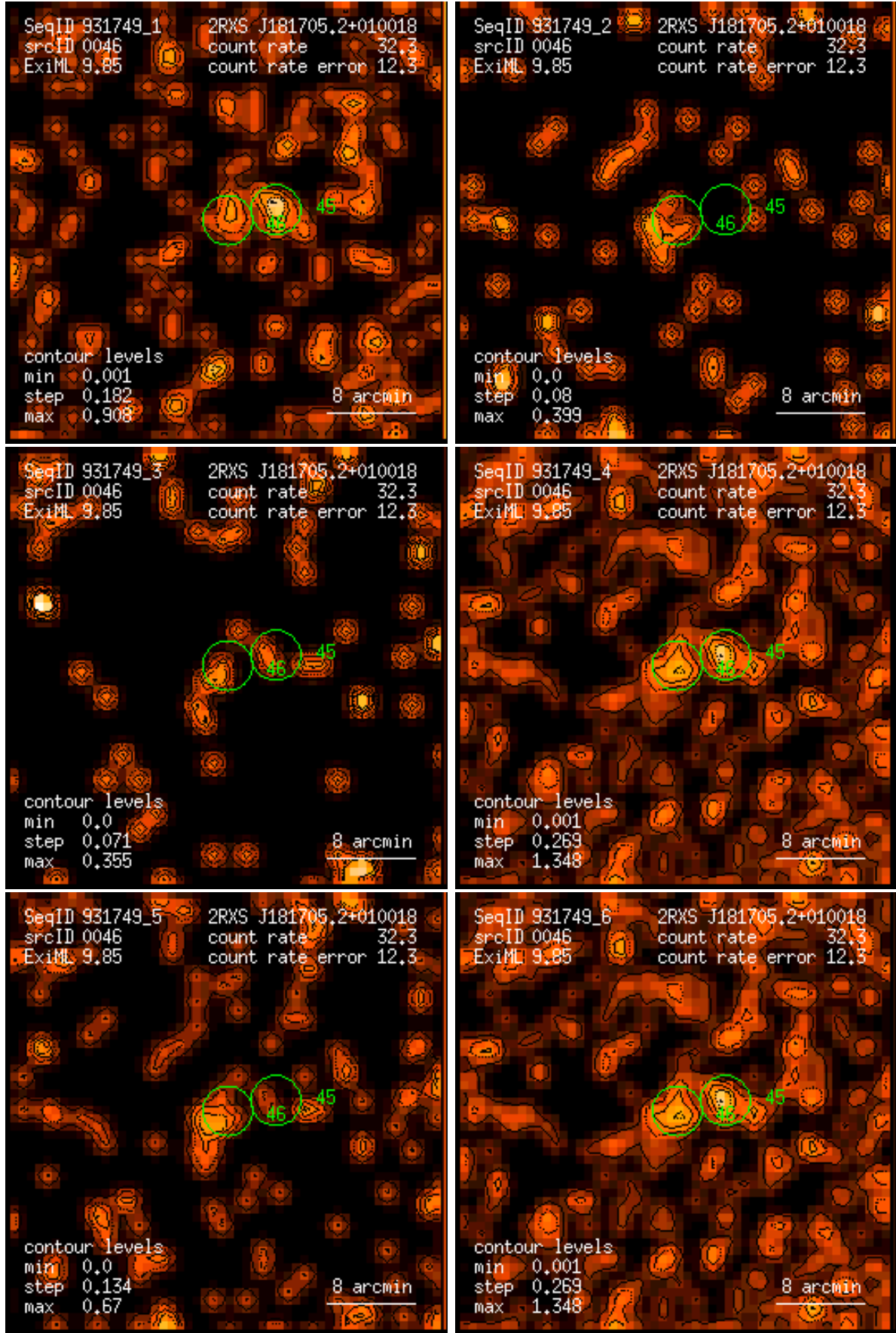
Figure 46: RASS 931749: detection 0046: band rate images, Gaussian filter: (1) PSPC channels 11 – 41, (2) 52 – 90, (3) 91 – 201, (4) 11 – 235, (5) 52 – 201, (6) 11 – 201. Broad band rates in counts/ks. Band rate contour levels in counts/ks/arcmin 2 .
