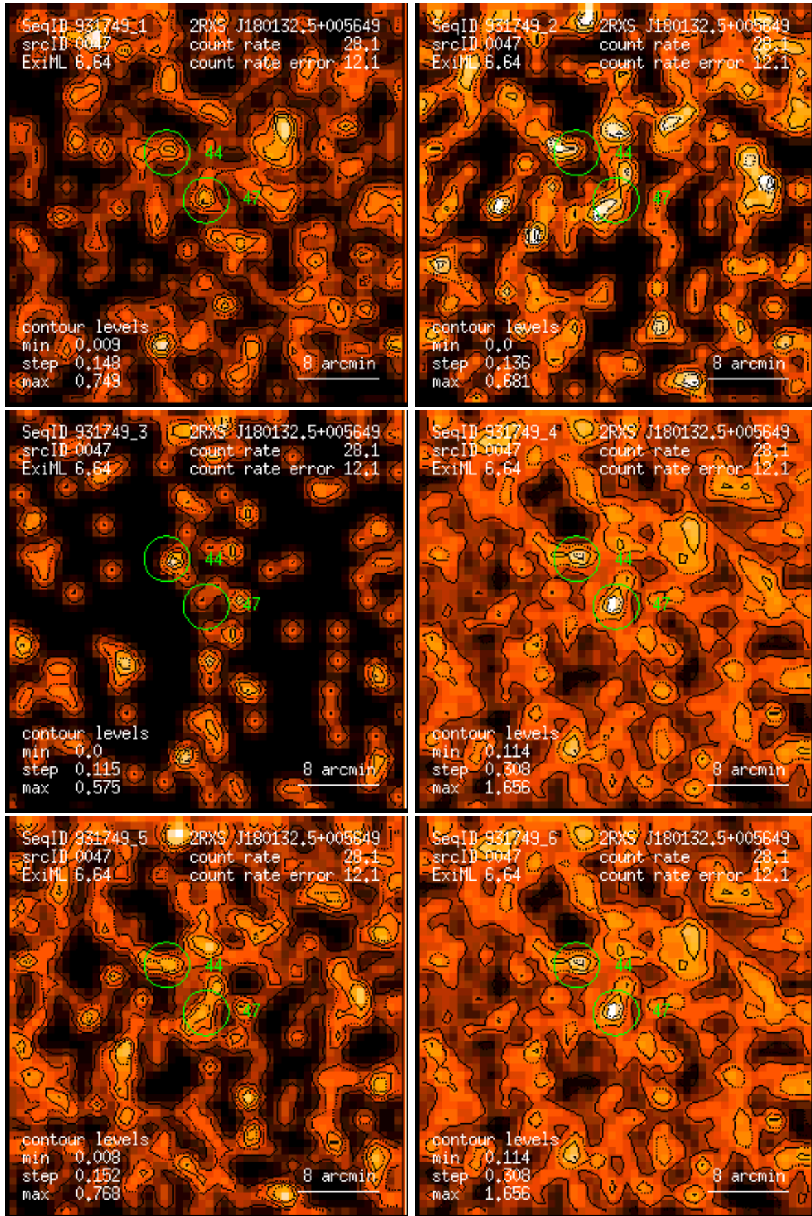
Figure 47: RASS 931749: detection 0047: band rate images, Gaussian filter: (1) PSPC channels 11 – 41, (2) 52 – 90, (3) 91 – 201, (4) 11 – 235, (5) 52 – 201, (6) 11 – 201. Broad band rates in counts/ks. Band rate contour levels in counts/ks/arcmin 2 .
