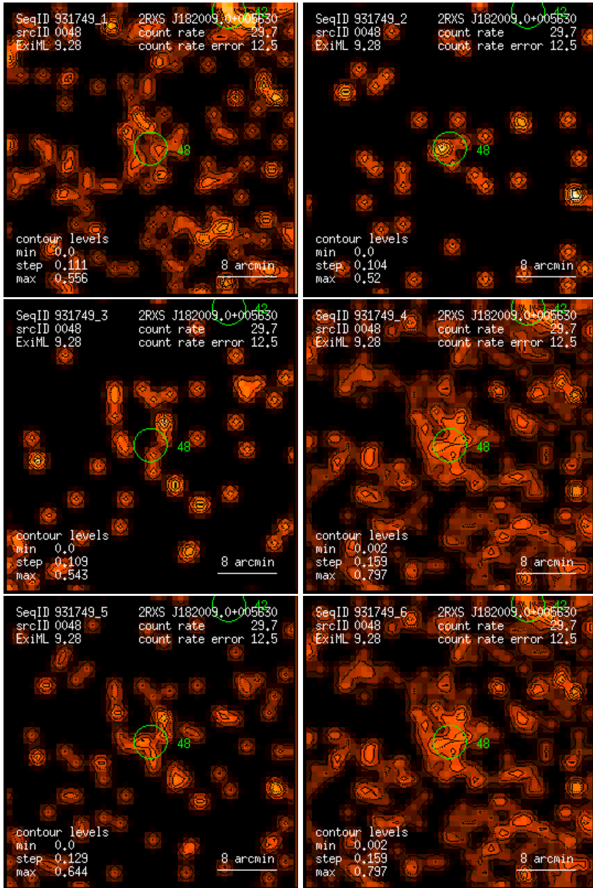
Figure 48: RASS 931749: detection 0048: band rate images, Gaussian filter: (1) PSPC channels 11 – 41, (2) 52 – 90, (3) 91 – 201, (4) 11 – 235, (5) 52 – 201, (6) 11 – 201. Broad band rates in counts/ks. Band rate contour levels in counts/ks/arcmin 2 .
