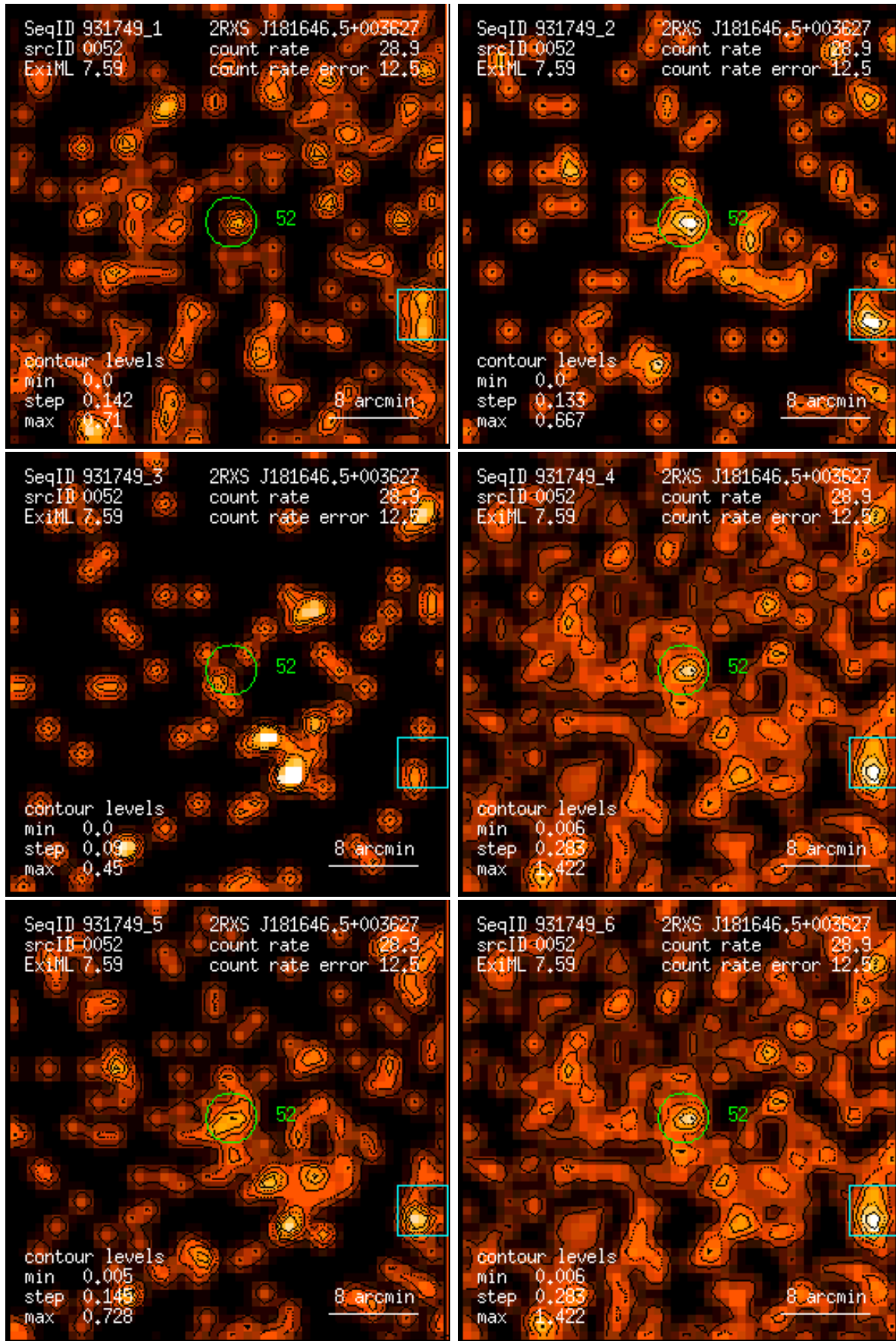
Figure 52: RASS 931749: detection 0052: band rate images, Gaussian filter: (1) PSPC channels 11 – 41, (2) 52 – 90, (3) 91 – 201, (4) 11 – 235, (5) 52 – 201, (6) 11 – 201. Broad band rates in counts/ks. Band rate contour levels in counts/ks/arcmin 2 .
