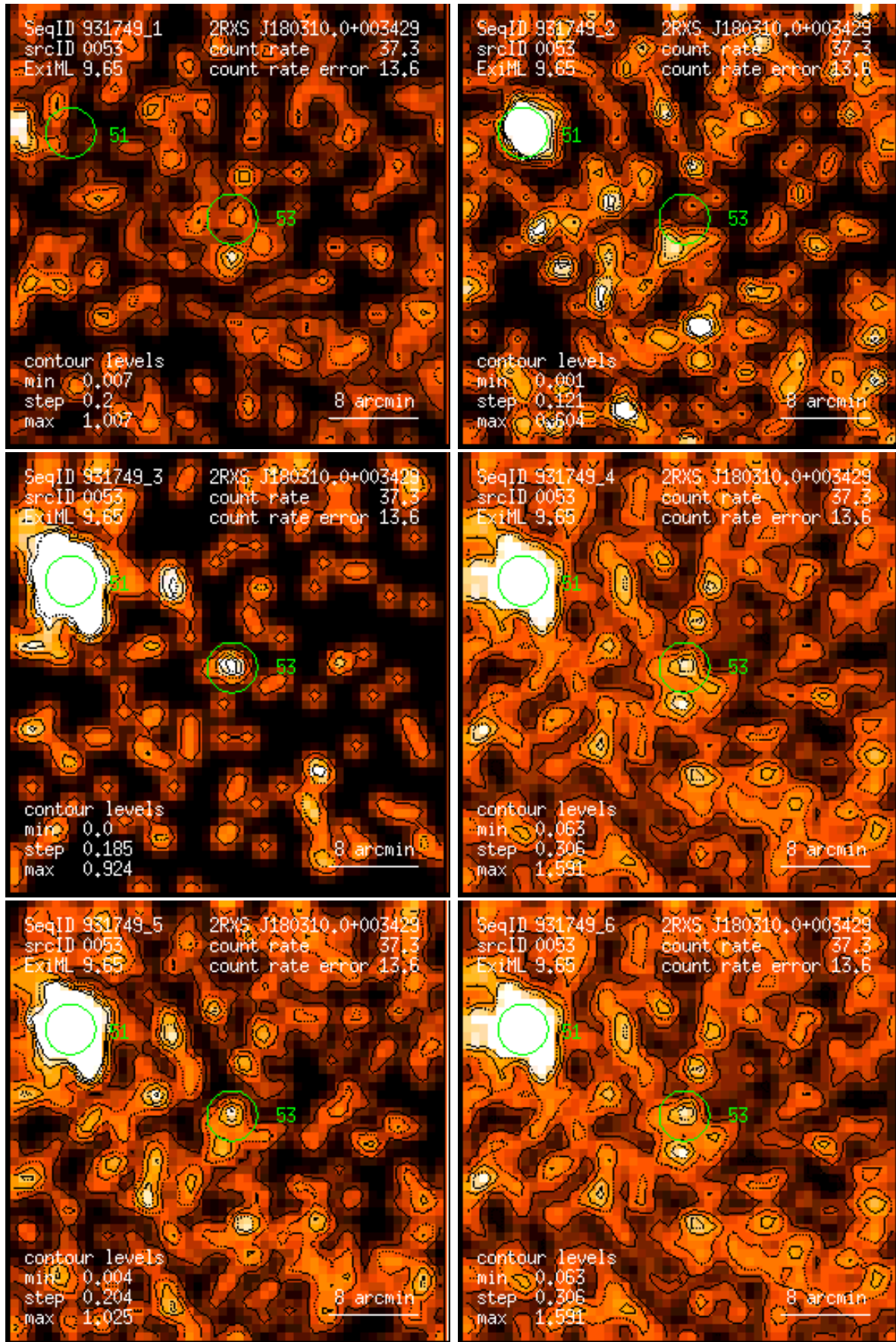
Figure 53: RASS 931749: detection 0053: band rate images, Gaussian filter: (1) PSPC channels 11 – 41, (2) 52 – 90, (3) 91 – 201, (4) 11 – 235, (5) 52 – 201, (6) 11 – 201. Broad band rates in counts/ks. Band rate contour levels in counts/ks/arcmin 2 .
