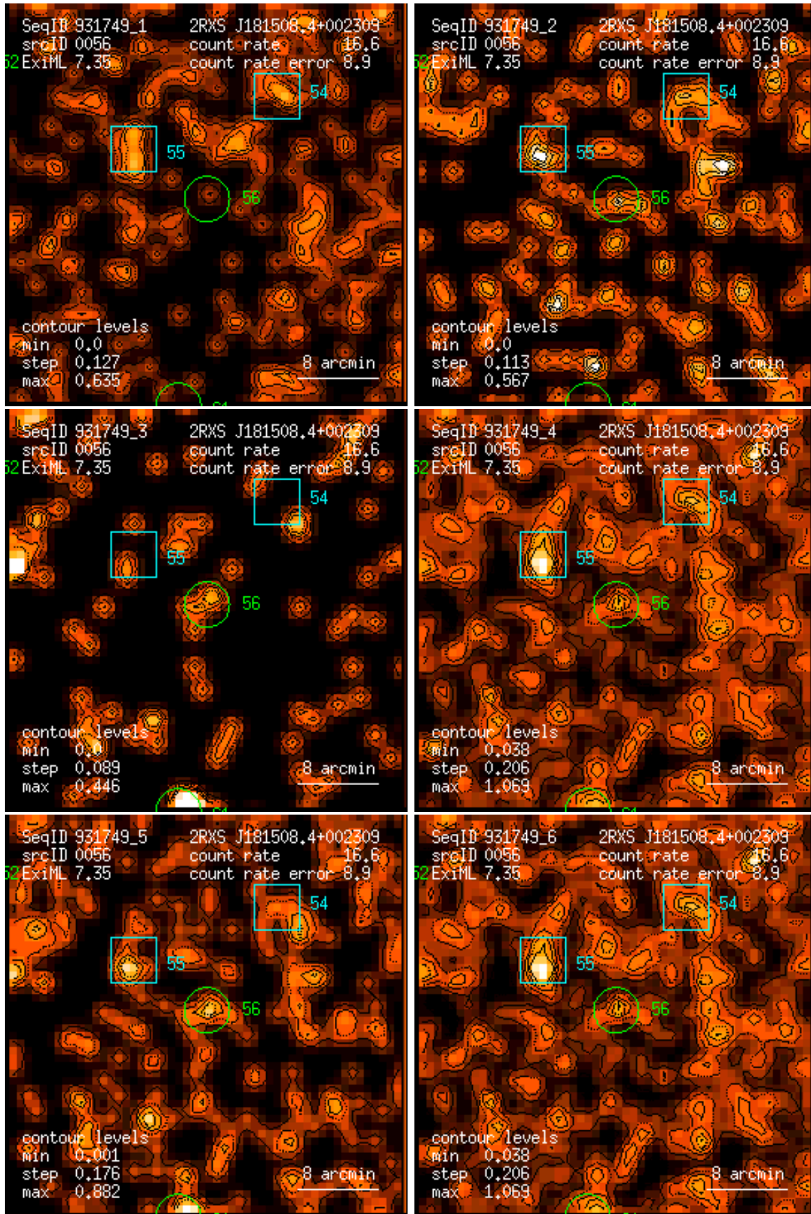
Figure 56: RASS 931749: detection 0056: band rate images, Gaussian filter: (1) PSPC channels 11 – 41, (2) 52 – 90, (3) 91 – 201, (4) 11 – 235, (5) 52 – 201, (6) 11 – 201. Broad band rates in counts/ks. Band rate contour levels in counts/ks/arcmin 2 .
