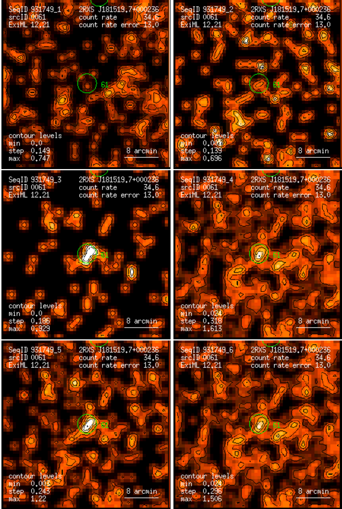
Figure 61: RASS 931749: detection 0061: band rate images, Gaussian filter: (1) PSPC channels 11 – 41, (2) 52 – 90, (3) 91 – 201, (4) 11 – 235, (5) 52 – 201, (6) 11 – 201. Broad band rates in counts/ks. Band rate contour levels in counts/ks/arcmin 2 .
