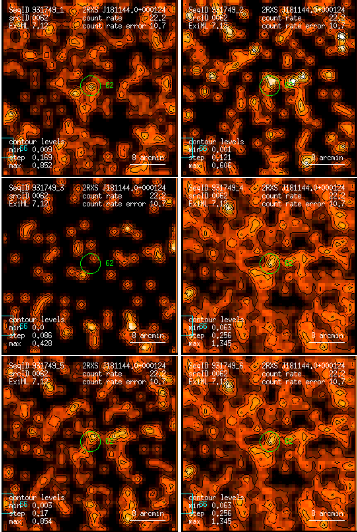
Figure 62: RASS 931749: detection 0062: band rate images, Gaussian filter: (1) PSPC channels 11 – 41, (2) 52 – 90, (3) 91 – 201, (4) 11 – 235, (5) 52 – 201, (6) 11 – 201. Broad band rates in counts/ks. Band rate contour levels in counts/ks/arcmin 2 .
