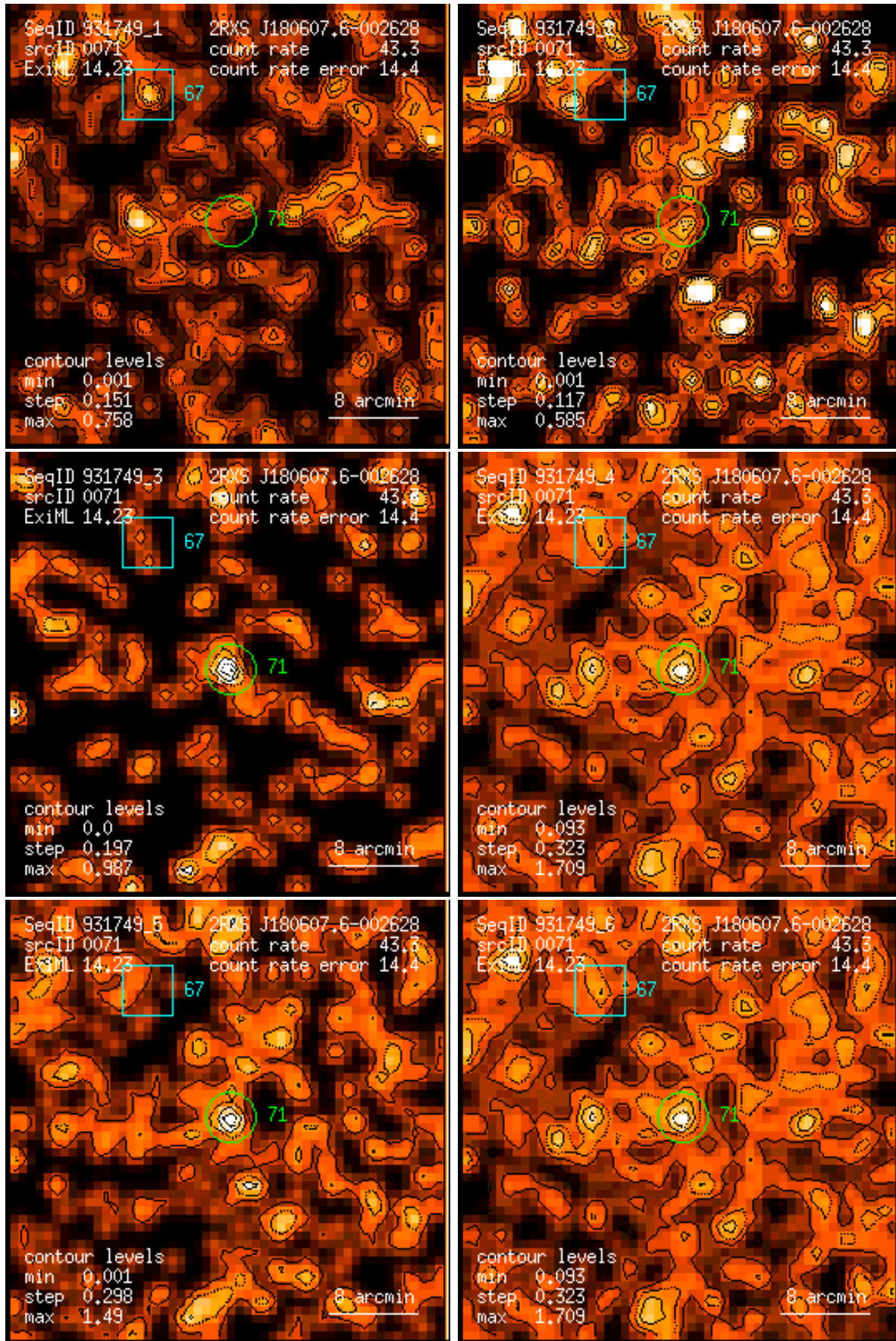
Figure 71: RASS 931749: detection 0071: band rate images, Gaussian filter: (1) PSPC channels 11 – 41, (2) 52 – 90, (3) 91 – 201, (4) 11 – 235, (5) 52 – 201, (6) 11 – 201. Broad band rates in counts/ks. Band rate contour levels in counts/ks/arcmin 2 .
