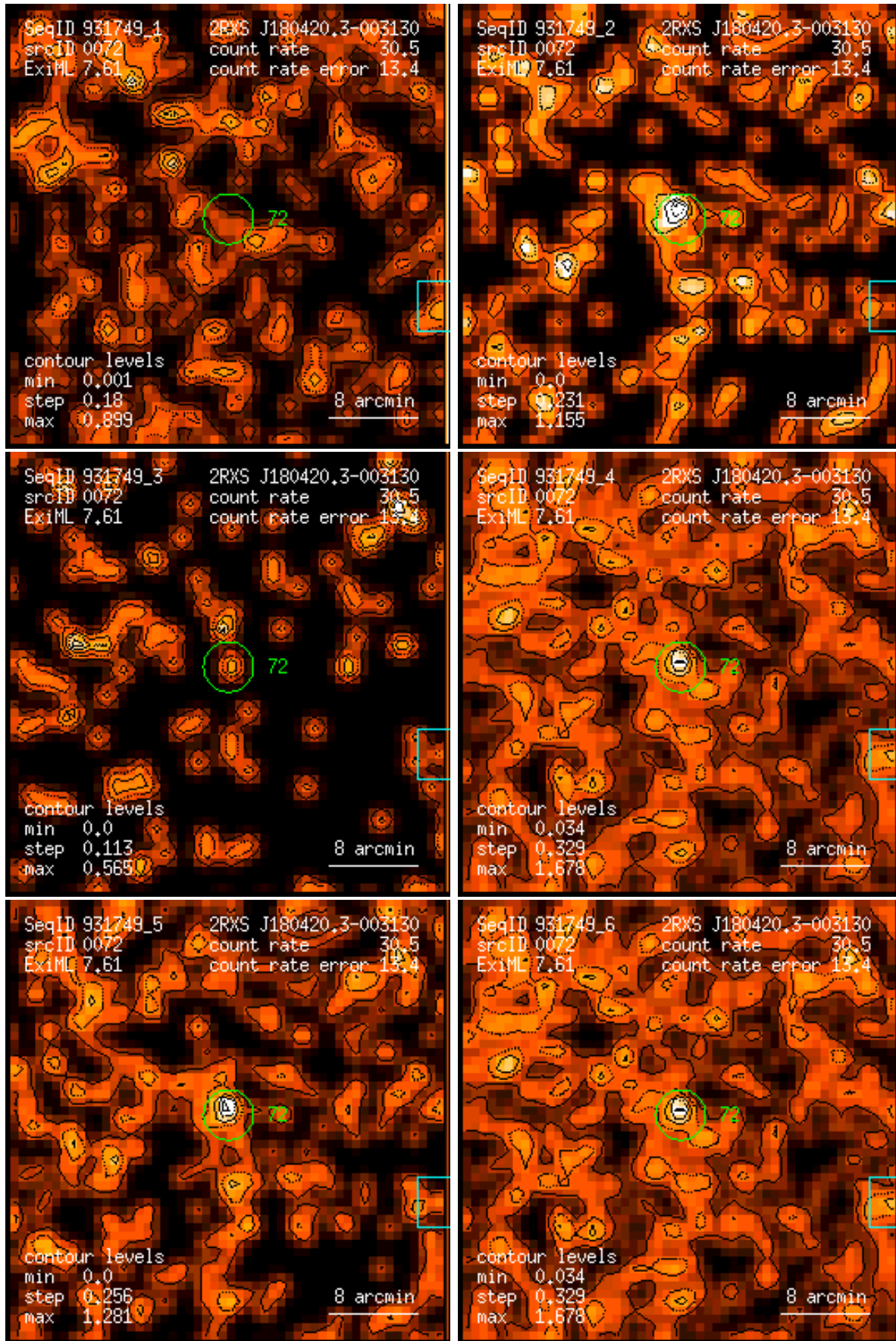
Figure 72: RASS 931749: detection 0072: band rate images, Gaussian filter: (1) PSPC channels 11 – 41, (2) 52 – 90, (3) 91 – 201, (4) 11 – 235, (5) 52 – 201, (6) 11 – 201. Broad band rates in counts/ks. Band rate contour levels in counts/ks/arcmin 2 .
