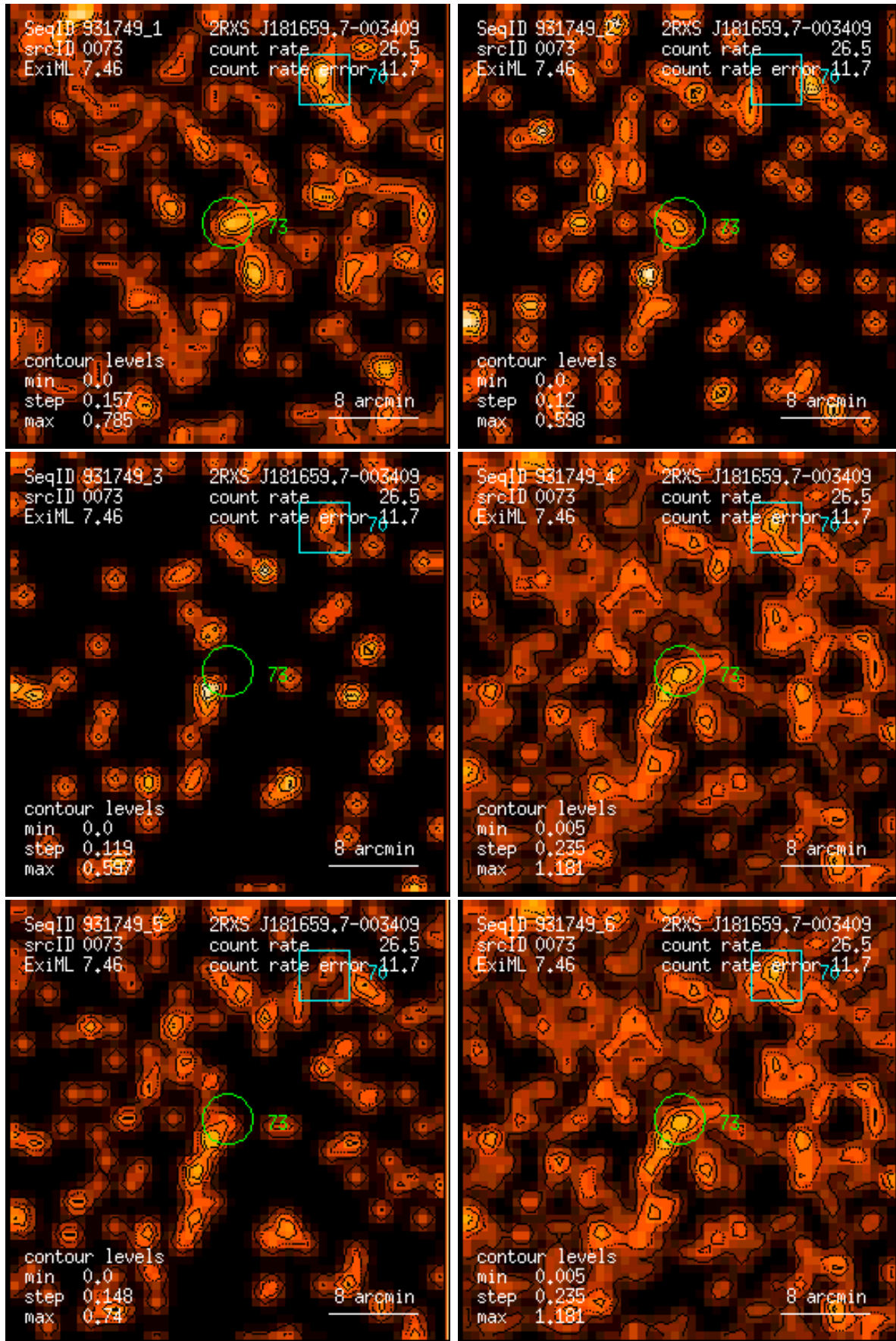
Figure 73: RASS 931749: detection 0073: band rate images, Gaussian filter: (1) PSPC channels 11 – 41, (2) 52 – 90, (3) 91 – 201, (4) 11 – 235, (5) 52 – 201, (6) 11 – 201. Broad band rates in counts/ks. Band rate contour levels in counts/ks/arcmin 2 .
