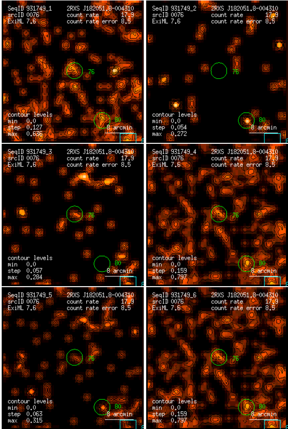
Figure 76: RASS 931749: detection 0076: band rate images, Gaussian filter: (1) PSPC channels 11 – 41, (2) 52 – 90, (3) 91 – 201, (4) 11 – 235, (5) 52 – 201, (6) 11 – 201. Broad band rates in counts/ks. Band rate contour levels in counts/ks/arcmin 2 .
