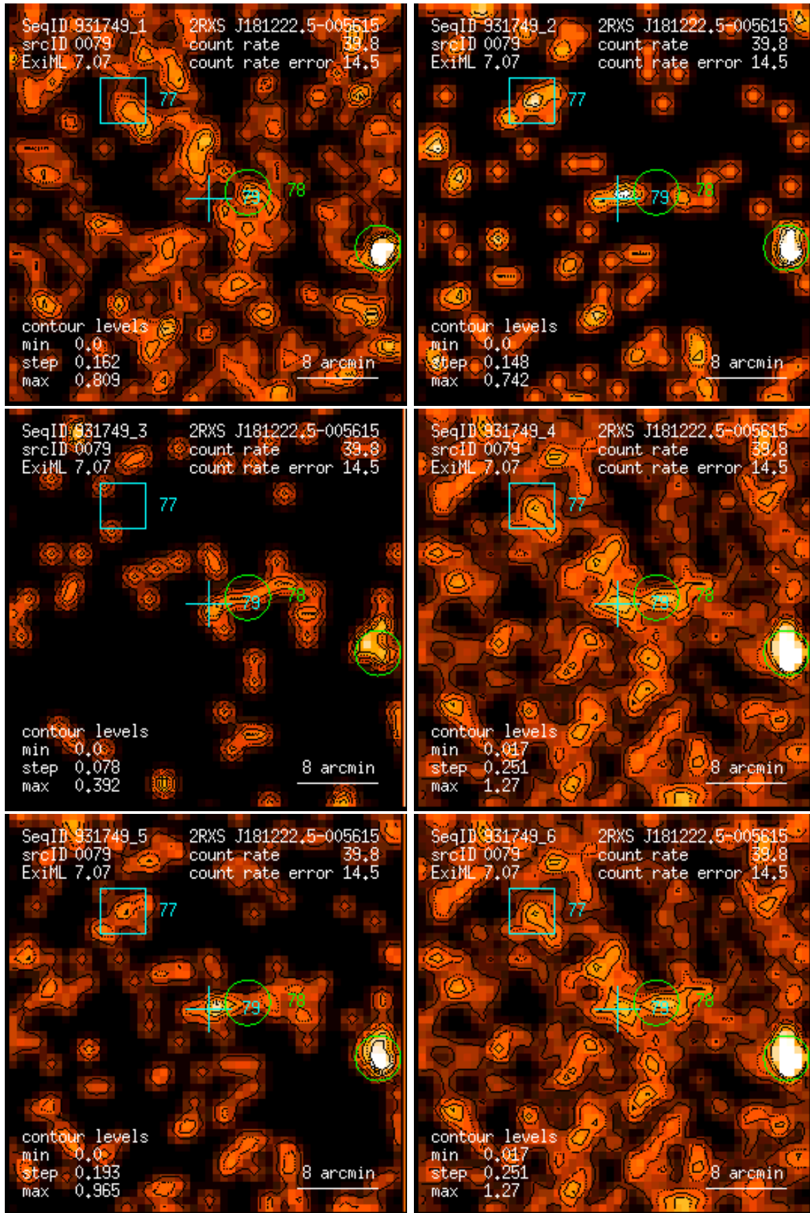
Figure 79: RASS 931749: detection 0079: band rate images, Gaussian filter: (1) PSPC channels 11 – 41, (2) 52 – 90, (3) 91 – 201, (4) 11 – 235, (5) 52 – 201, (6) 11 – 201. Broad band rates in counts/ks. Band rate contour levels in counts/ks/arcmin 2 .
