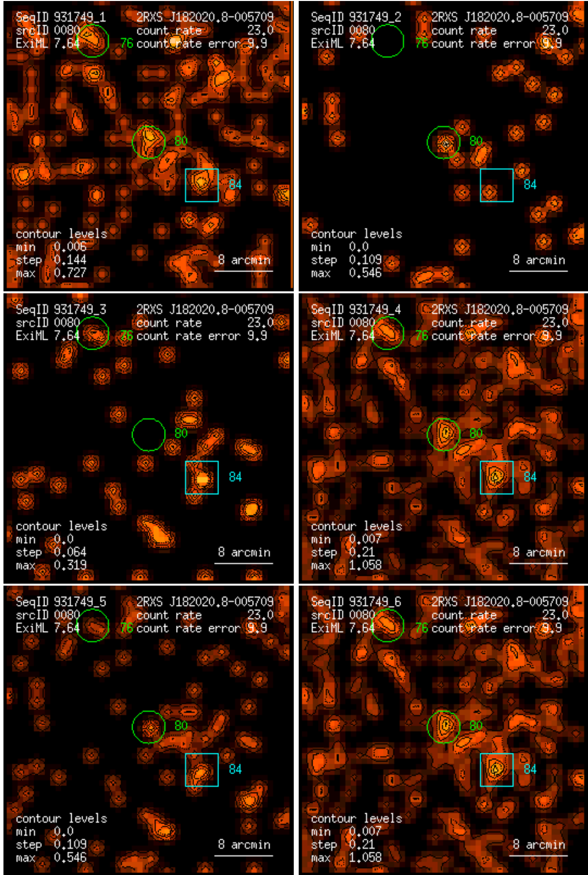
Figure 80: RASS 931749: detection 0080: band rate images, Gaussian filter: (1) PSPC channels 11 – 41, (2) 52 – 90, (3) 91 – 201, (4) 11 – 235, (5) 52 – 201, (6) 11 – 201. Broad band rates in counts/ks. Band rate contour levels in counts/ks/arcmin 2 .
