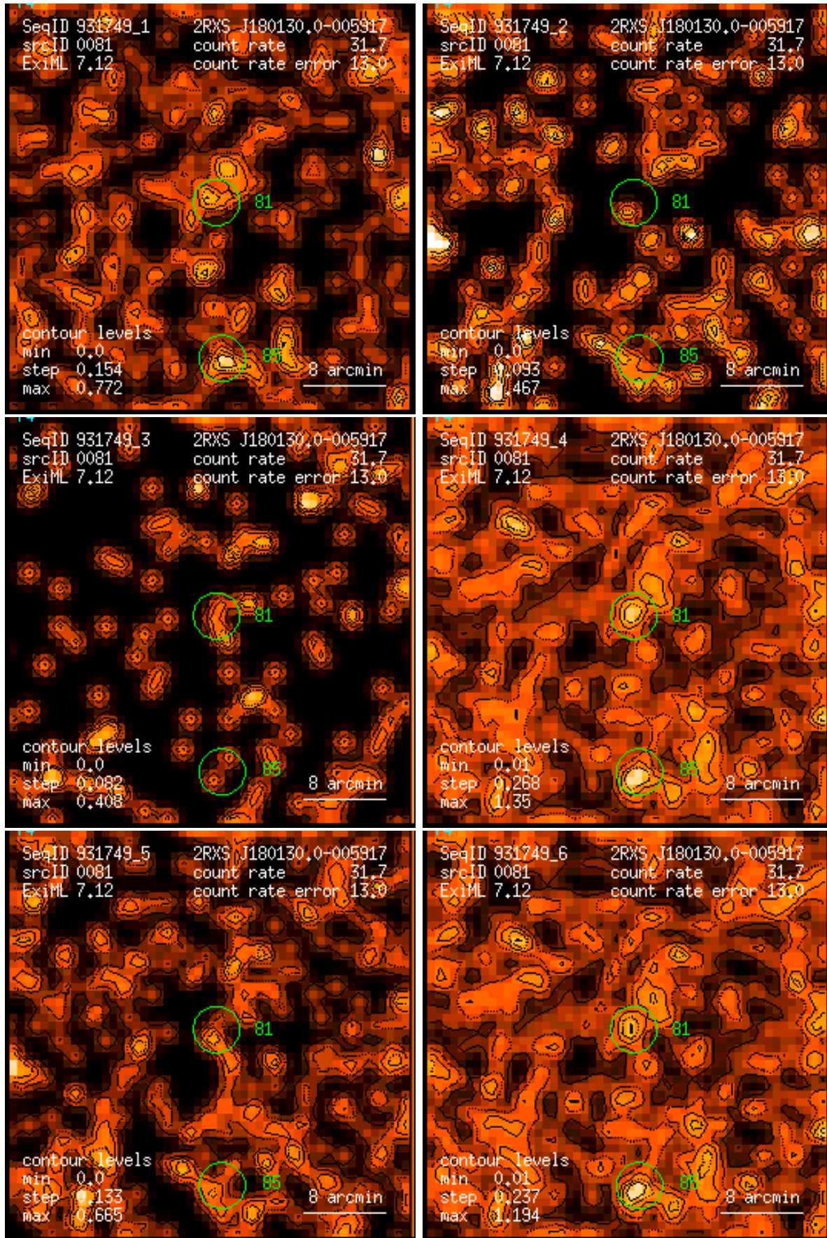
Figure 81: RASS 931749: detection 0081: band rate images, Gaussian filter: (1) PSPC channels 11 – 41, (2) 52 – 90, (3) 91 – 201, (4) 11 – 235, (5) 52 – 201, (6) 11 – 201. Broad band rates in counts/ks. Band rate contour levels in counts/ks/arcmin 2 .
